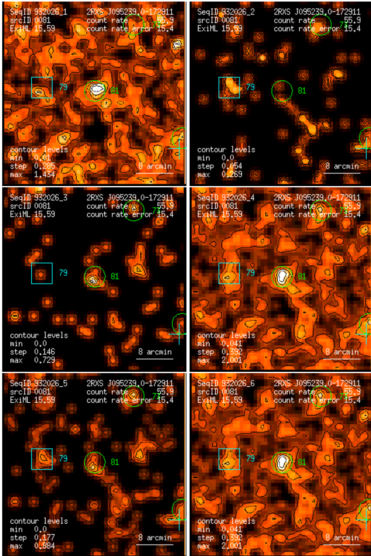
Figure 81: RASS 932026: detection 0081: band rate images, Gaussian filter: (1) PSPC channels 11 – 41, (2) 52 – 90, (3) 91 – 201, (4) 11 – 235, (5) 52 – 201, (6) 11 – 201. Broad band rates in counts/ks. Band rate contour levels in counts/ks/arcmin 2 .
