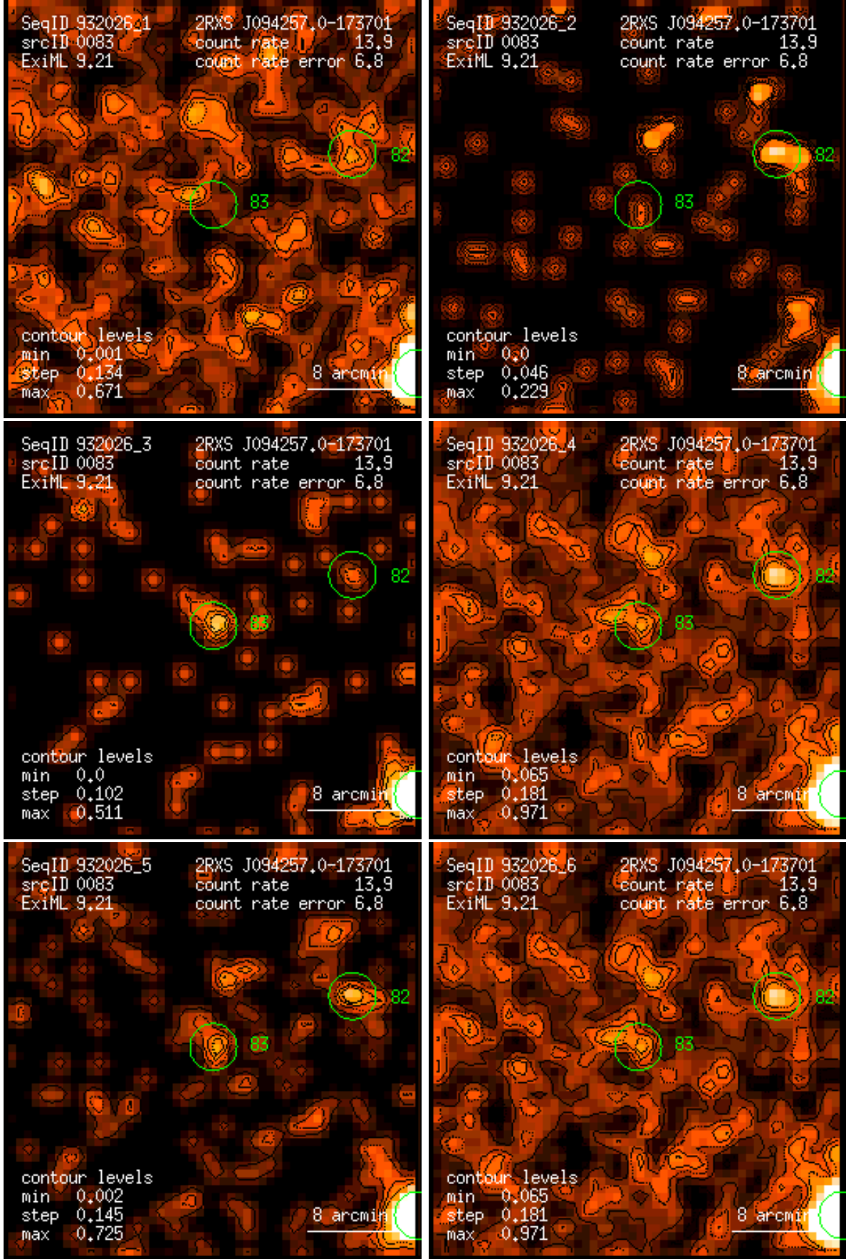
Figure 83: RASS 932026: detection 0083: band rate images, Gaussian filter: (1) PSPC channels 11 – 41, (2) 52 – 90, (3) 91 – 201, (4) 11 – 235, (5) 52 – 201, (6) 11 – 201. Broad band rates in counts/ks. Band rate contour levels in counts/ks/arcmin 2 .
