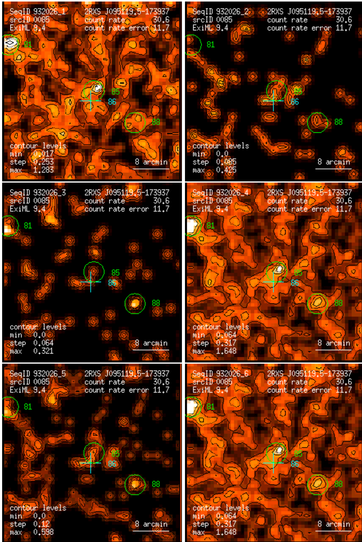
Figure 85: RASS 932026: detection 0085: band rate images, Gaussian filter: (1) PSPC channels 11 – 41, (2) 52 – 90, (3) 91 – 201, (4) 11 – 235, (5) 52 – 201, (6) 11 – 201. Broad band rates in counts/ks. Band rate contour levels in counts/ks/arcmin 2 .
