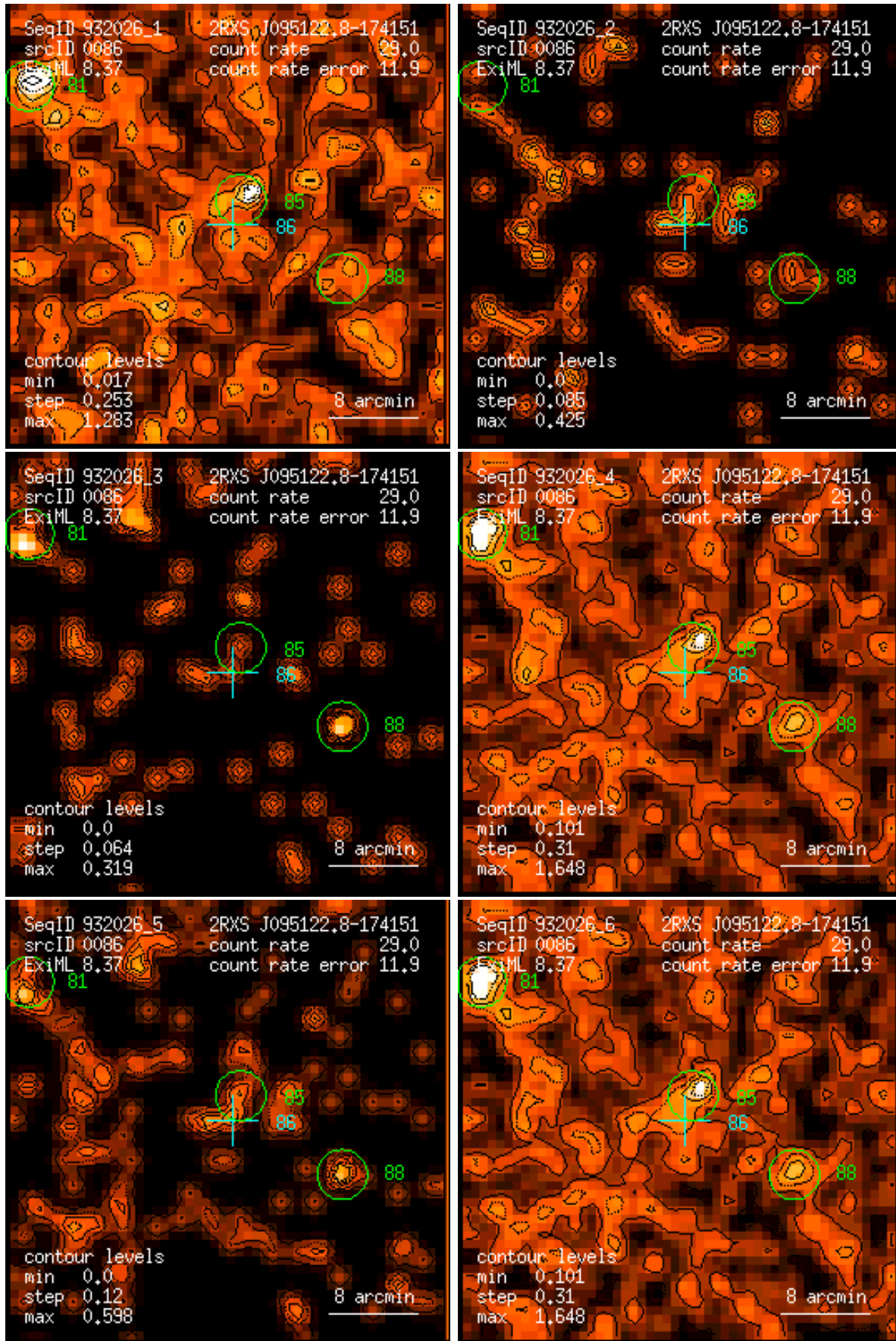
Figure 86: RASS 932026: detection 0086: band rate images, Gaussian filter: (1) PSPC channels 11 – 41, (2) 52 – 90, (3) 91 – 201, (4) 11 – 235, (5) 52 – 201, (6) 11 – 201. Broad band rates in counts/ks. Band rate contour levels in counts/ks/arcmin 2 .
