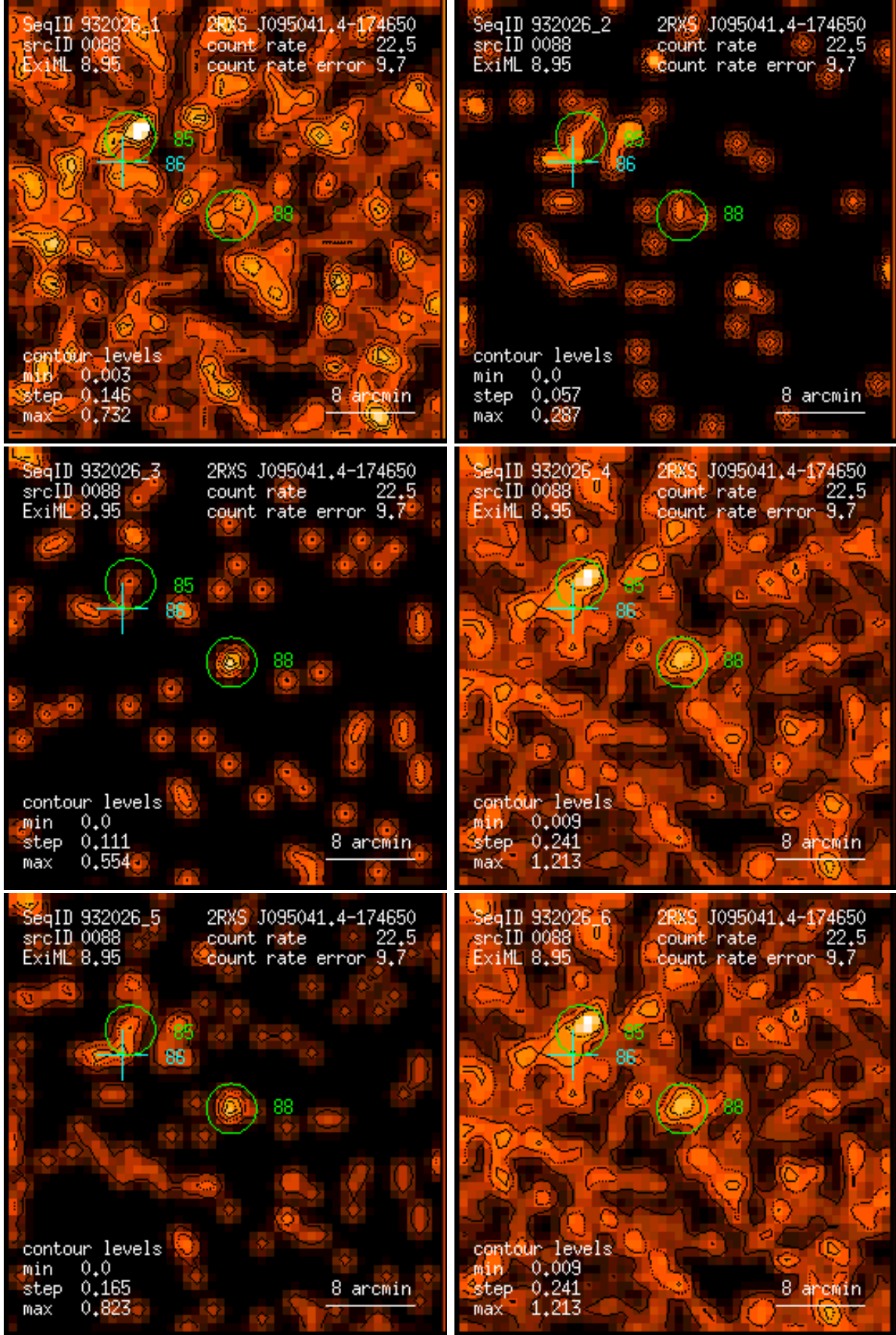
Figure 88: RASS 932026: detection 0088: band rate images, Gaussian filter: (1) PSPC channels 11 – 41, (2) 52 – 90, (3) 91 – 201, (4) 11 – 235, (5) 52 – 201, (6) 11 – 201. Broad band rates in counts/ks. Band rate contour levels in counts/ks/arcmin 2 .
