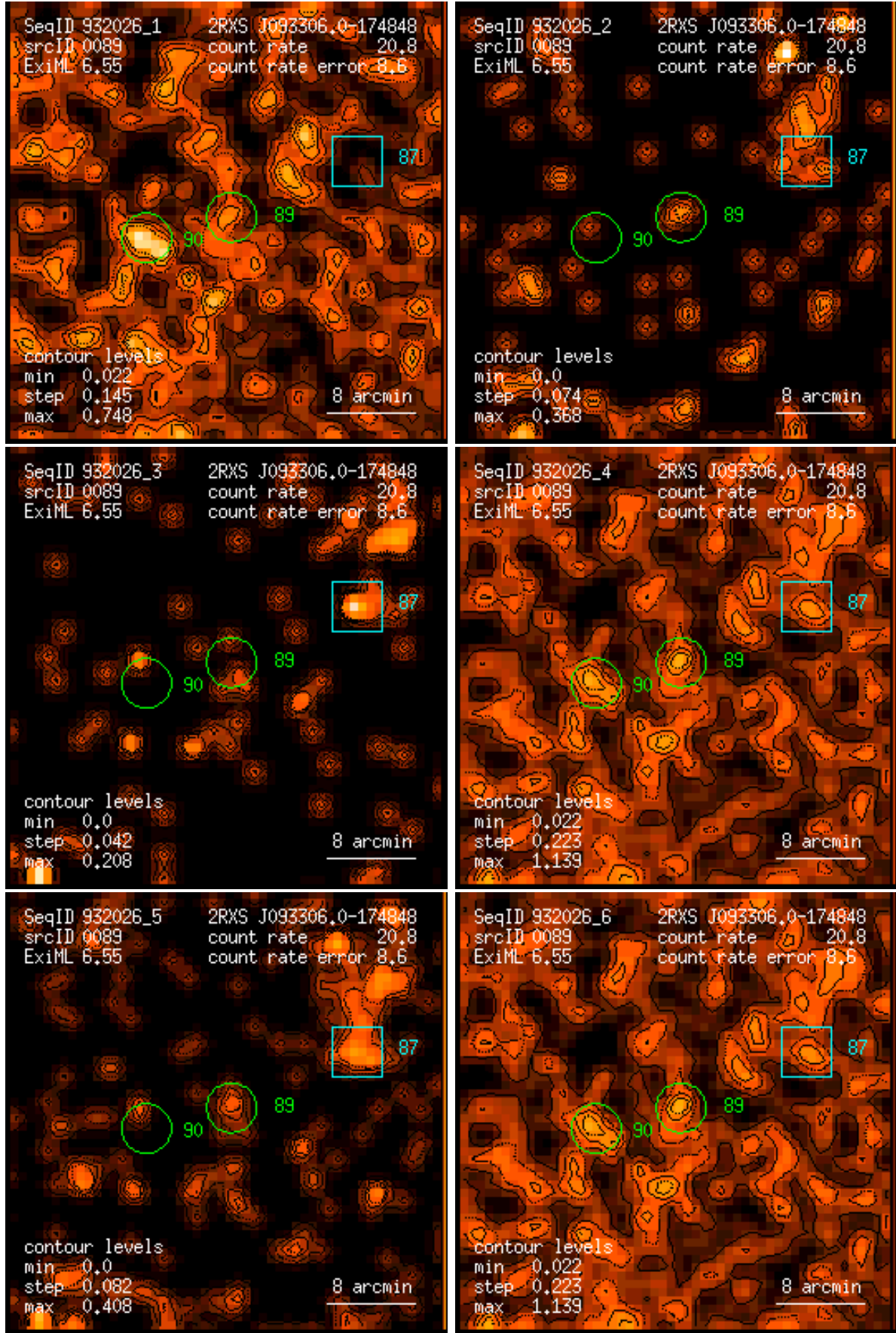
Figure 89: RASS 932026: detection 0089: band rate images, Gaussian filter: (1) PSPC channels 11 – 41, (2) 52 – 90, (3) 91 – 201, (4) 11 – 235, (5) 52 – 201, (6) 11 – 201. Broad band rates in counts/ks. Band rate contour levels in counts/ks/arcmin 2 .
