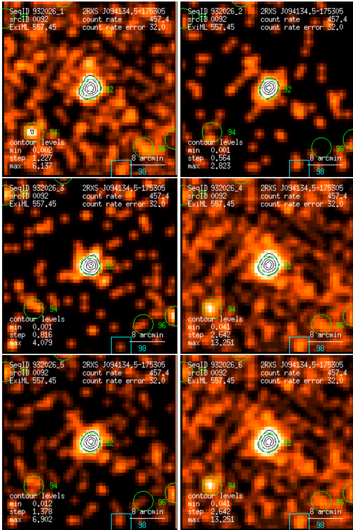
Figure 92: RASS 932026: detection 0092: band rate images, Gaussian filter: (1) PSPC channels 11 – 41, (2) 52 – 90, (3) 91 – 201, (4) 11 – 235, (5) 52 – 201, (6) 11 – 201. Broad band rates in counts/ks. Band rate contour levels in counts/ks/arcmin 2 .
