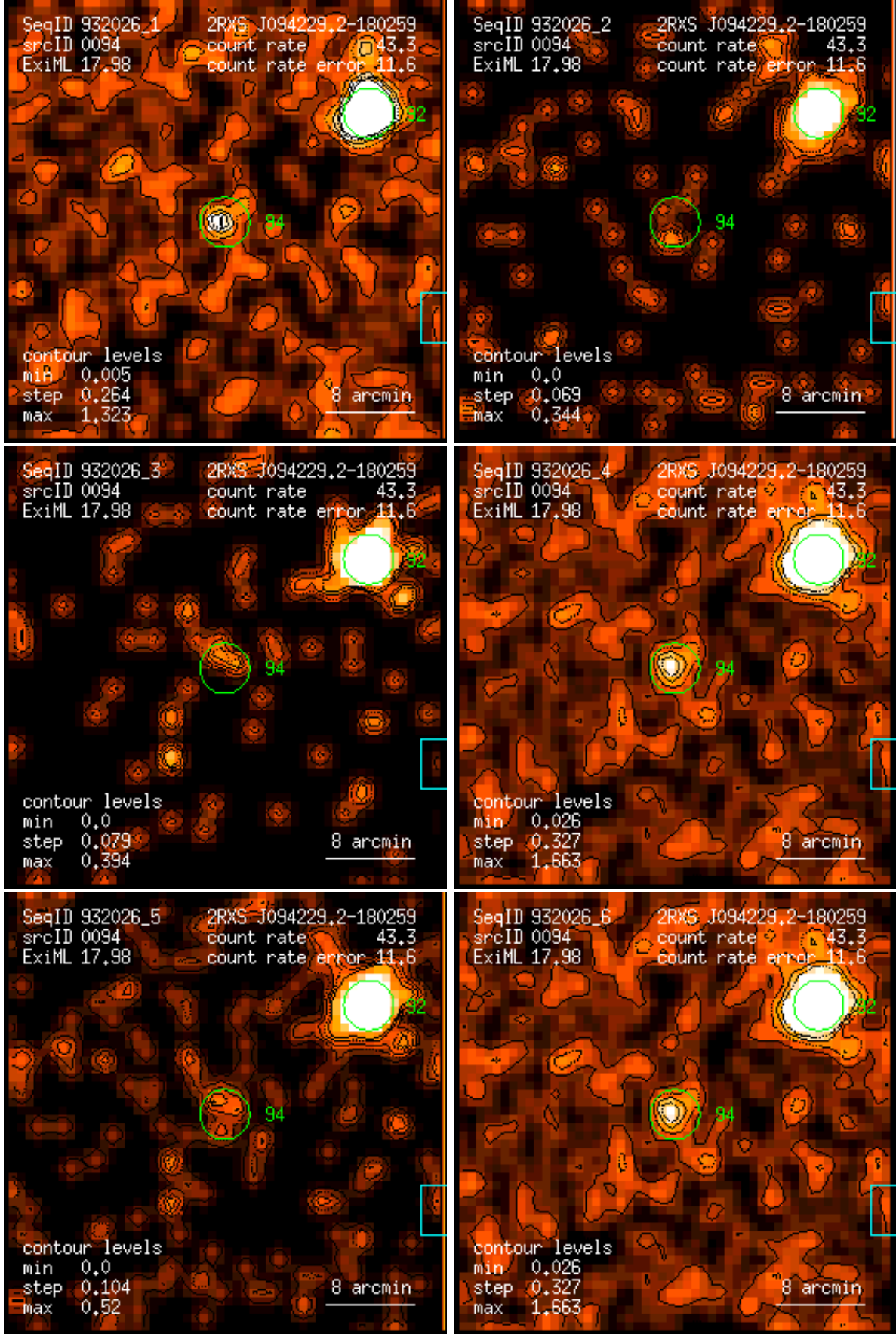
Figure 94: RASS 932026: detection 0094: band rate images, Gaussian filter: (1) PSPC channels 11 – 41, (2) 52 – 90, (3) 91 – 201, (4) 11 – 235, (5) 52 – 201, (6) 11 – 201. Broad band rates in counts/ks. Band rate contour levels in counts/ks/arcmin 2 .
