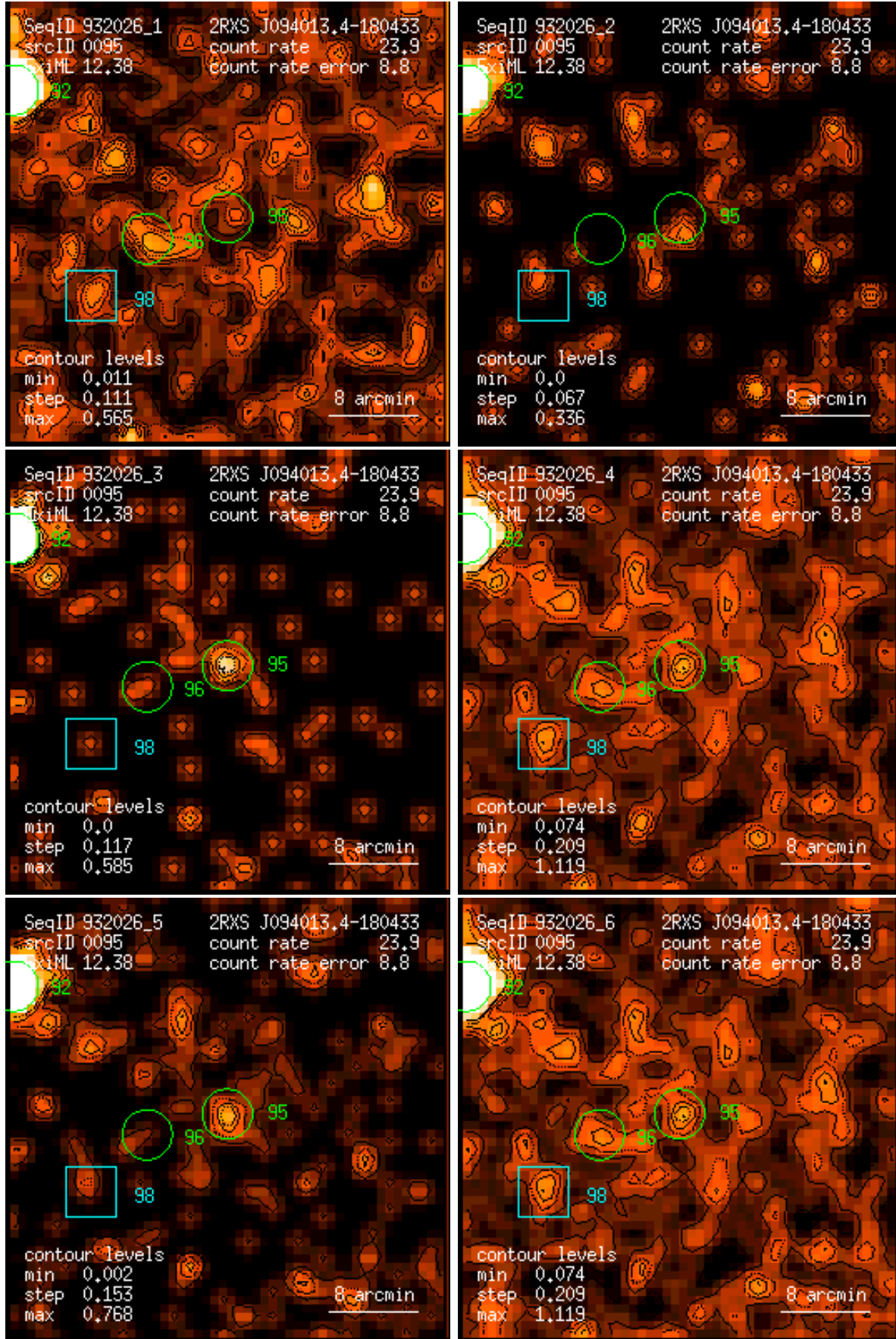
Figure 95: RASS 932026: detection 0095: band rate images, Gaussian filter: (1) PSPC channels 11 – 41, (2) 52 – 90, (3) 91 – 201, (4) 11 – 235, (5) 52 – 201, (6) 11 – 201. Broad band rates in counts/ks. Band rate contour levels in counts/ks/arcmin 2 .
