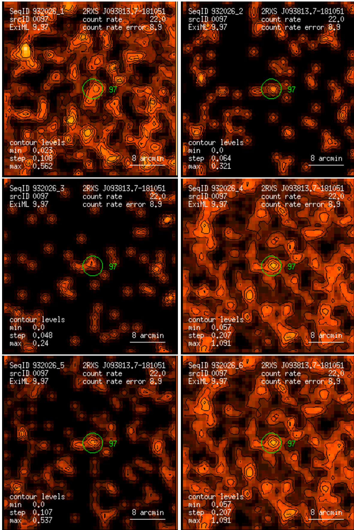
Figure 97: RASS 932026: detection 0097: band rate images, Gaussian filter: (1) PSPC channels 11 – 41, (2) 52 – 90, (3) 91 – 201, (4) 11 – 235, (5) 52 – 201, (6) 11 – 201. Broad band rates in counts/ks. Band rate contour levels in counts/ks/arcmin 2 .
