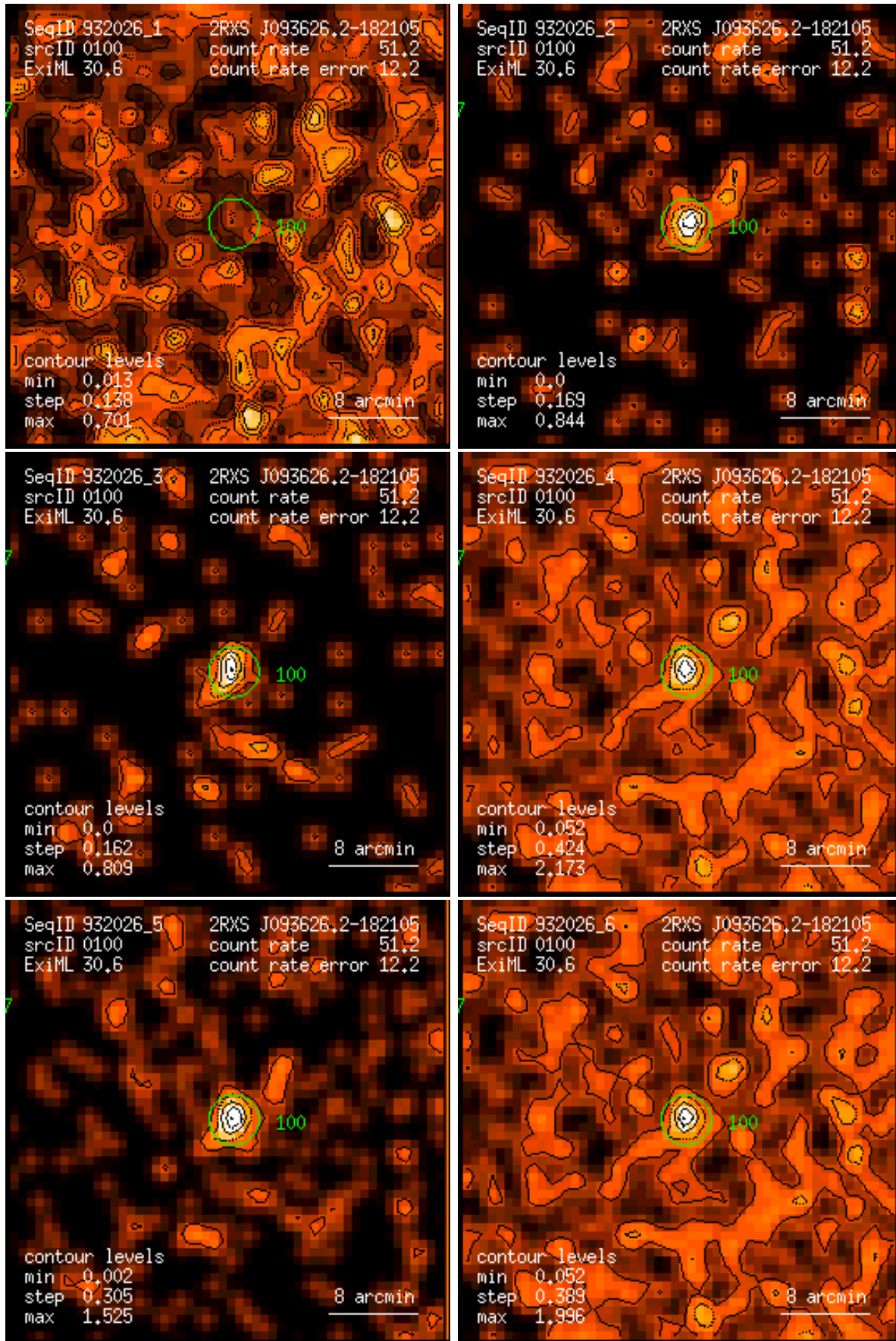
Figure 100: RASS 932026: detection 0100: band rate images, Gaussian filter: (1) PSPC channels 11 – 41, (2) 52 – 90, (3) 91 – 201, (4) 11 – 235, (5) 52 – 201, (6) 11 – 201. Broad band rates in counts/ks. Band rate contour levels in counts/ks/arcmin 2 .
