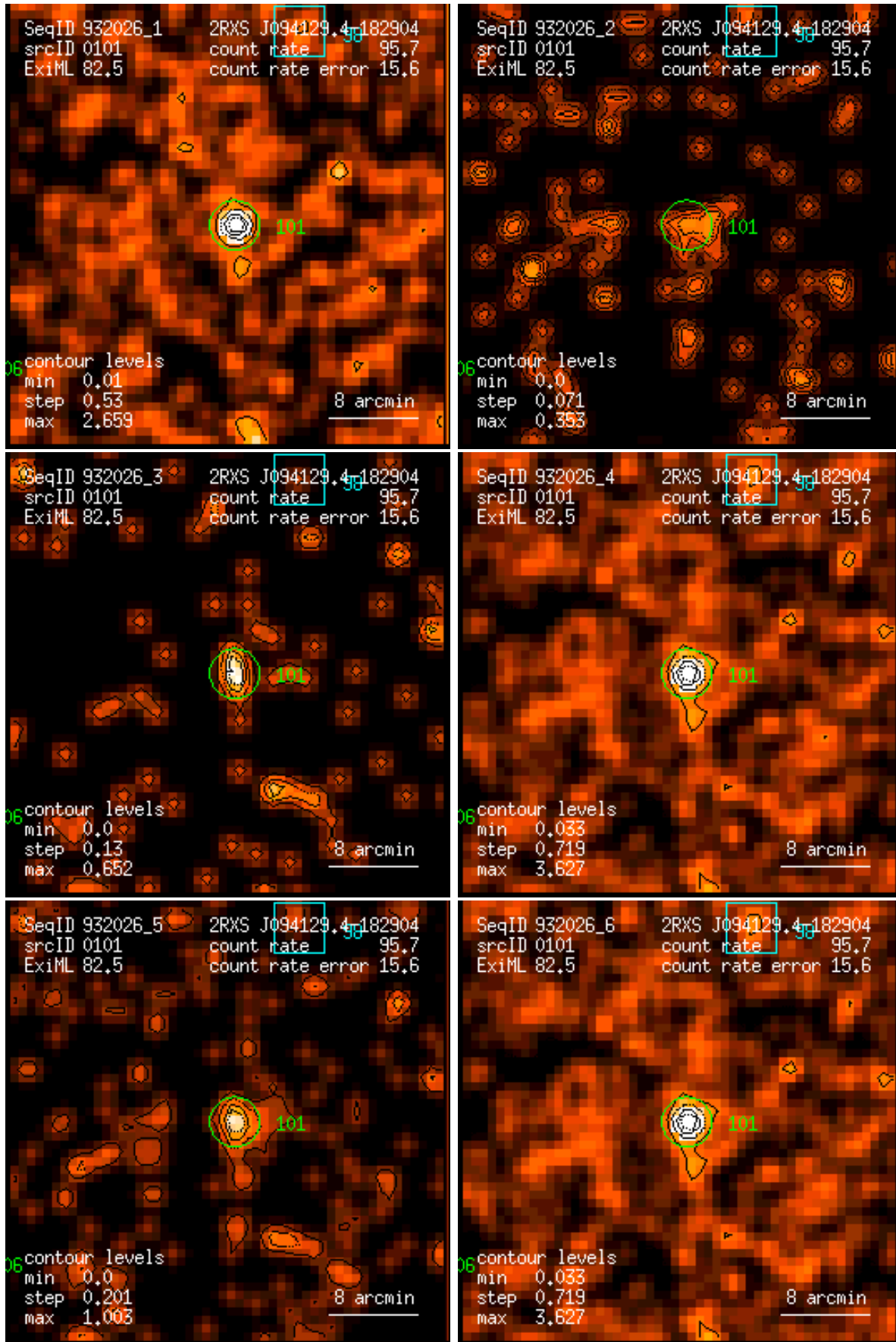
Figure 101: RASS 932026: detection 0101: band rate images, Gaussian filter: (1) PSPC channels 11 – 41, (2) 52 – 90, (3) 91 – 201, (4) 11 – 235, (5) 52 – 201, (6) 11 – 201. Broad band rates in counts/ks. Band rate contour levels in counts/ks/arcmin 2 .
