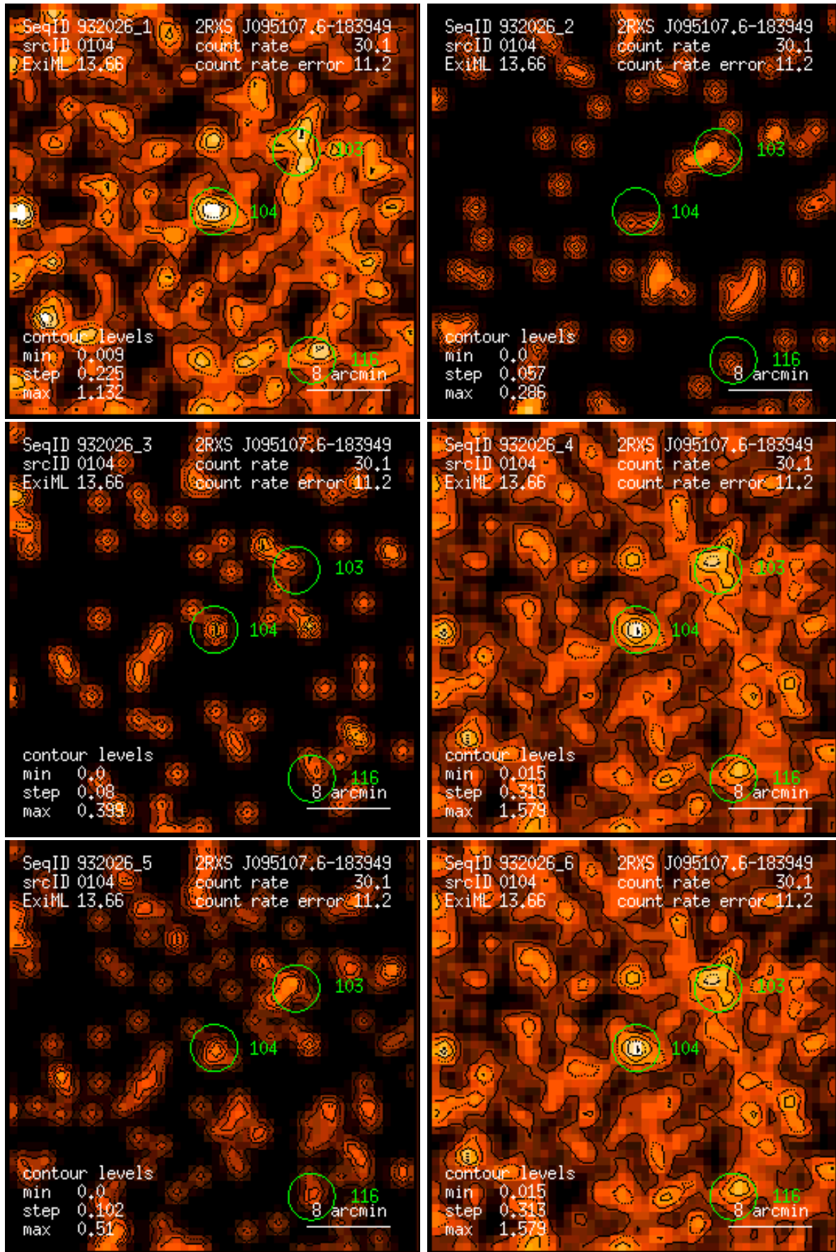
Figure 104: RASS 932026: detection 0104: band rate images, Gaussian filter: (1) PSPC channels 11 – 41, (2) 52 – 90, (3) 91 – 201, (4) 11 – 235, (5) 52 – 201, (6) 11 – 201. Broad band rates in counts/ks. Band rate contour levels in counts/ks/arcmin 2 .
