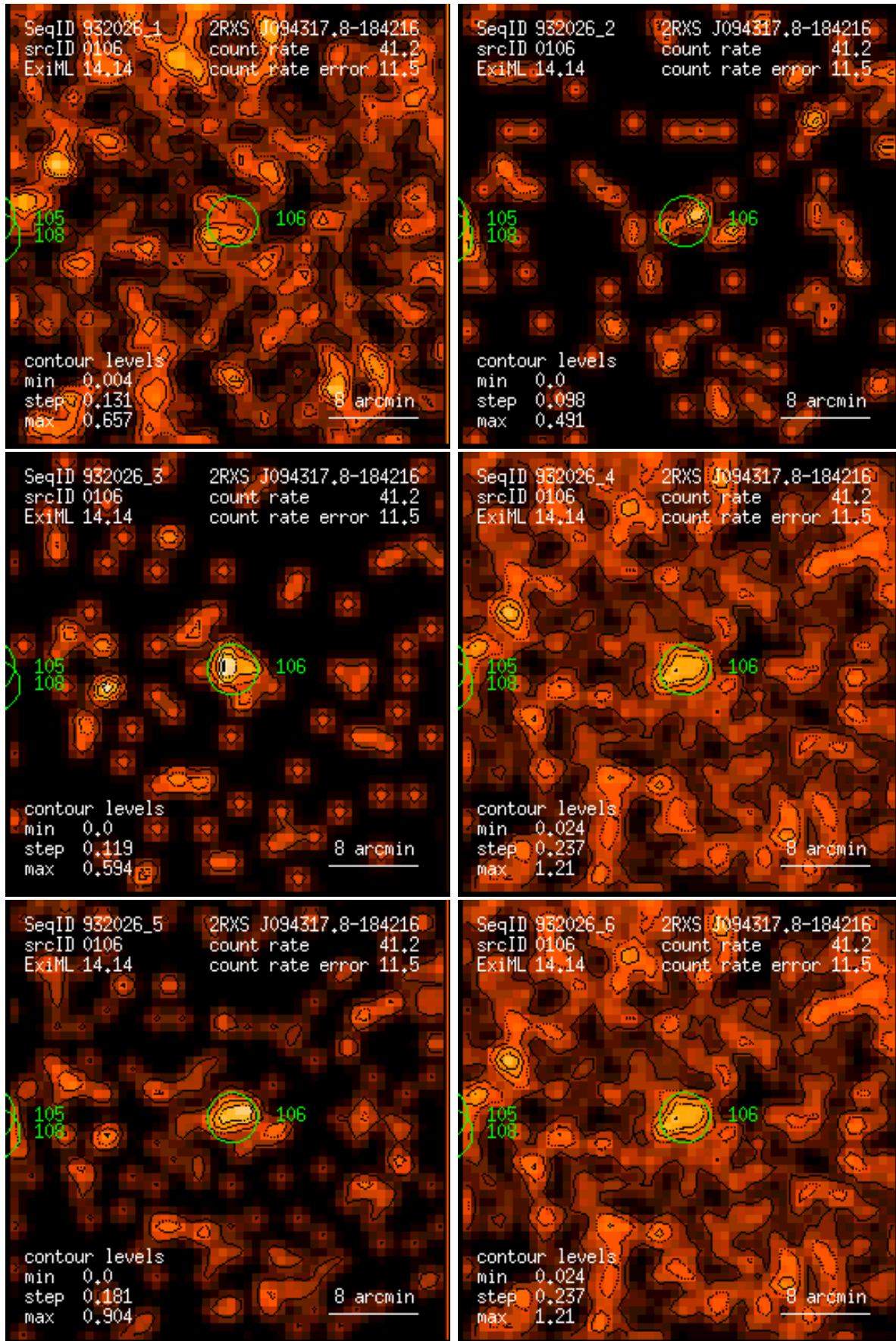
Figure 106: RASS 932026: detection 0106: band rate images, Gaussian filter: (1) PSPC channels 11 – 41, (2) 52 – 90, (3) 91 – 201, (4) 11 – 235, (5) 52 – 201, (6) 11 – 201. Broad band rates in counts/ks. Band rate contour levels in counts/ks/arcmin 2 .
