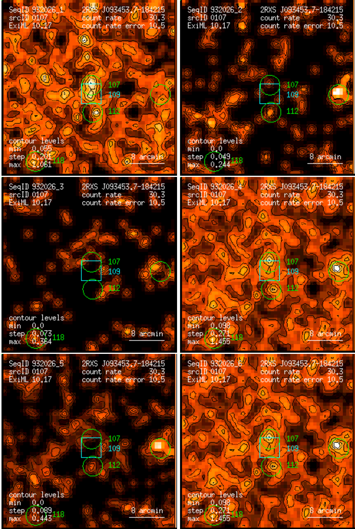
Figure 107: RASS 932026: detection 0107: band rate images, Gaussian filter: (1) PSPC channels 11 – 41, (2) 52 – 90, (3) 91 – 201, (4) 11 – 235, (5) 52 – 201, (6) 11 – 201. Broad band rates in counts/ks. Band rate contour levels in counts/ks/arcmin 2 .
