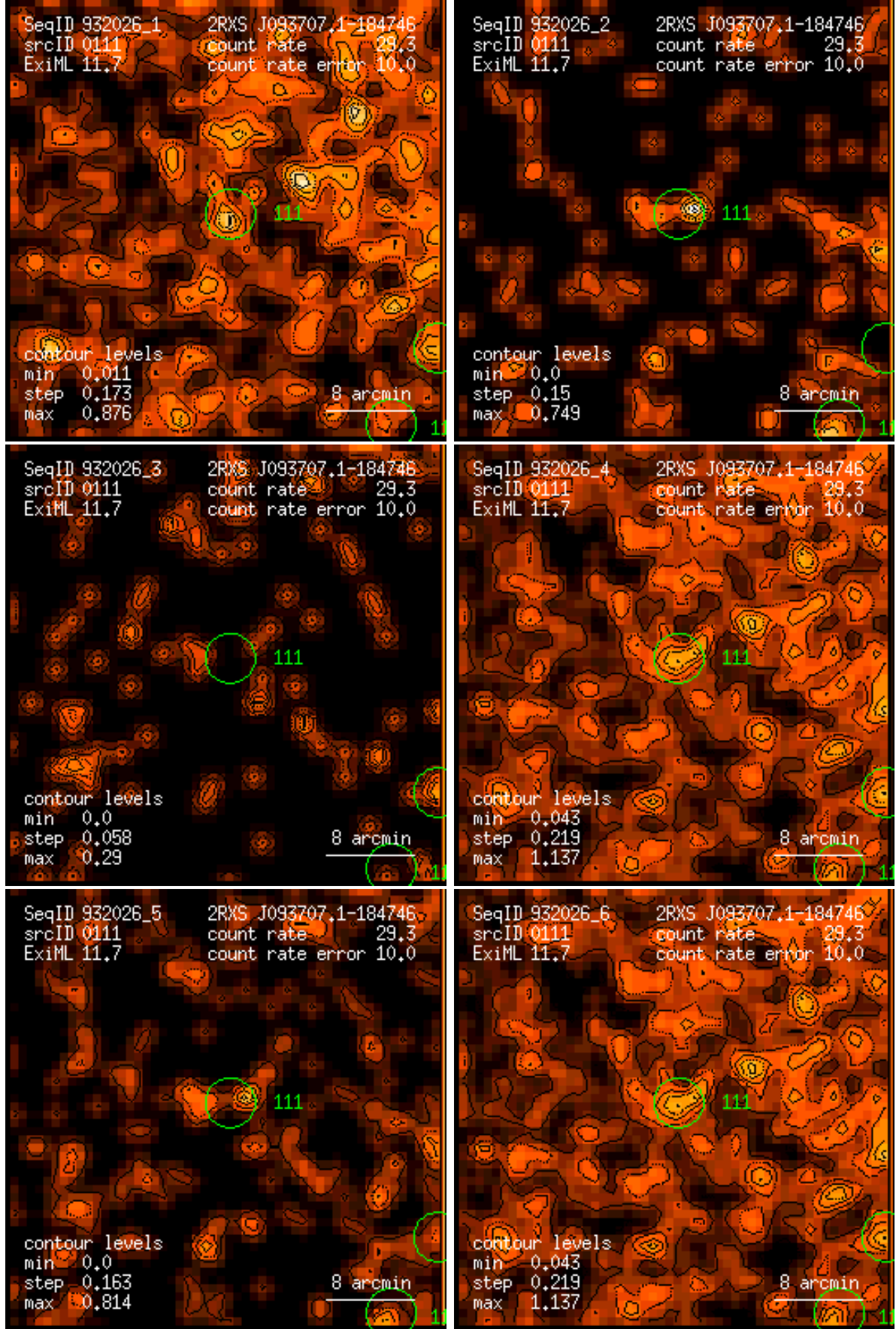
Figure 111: RASS 932026: detection 0111: band rate images, Gaussian filter: (1) PSPC channels 11 – 41, (2) 52 – 90, (3) 91 – 201, (4) 11 – 235, (5) 52 – 201, (6) 11 – 201. Broad band rates in counts/ks. Band rate contour levels in counts/ks/arcmin 2 .
