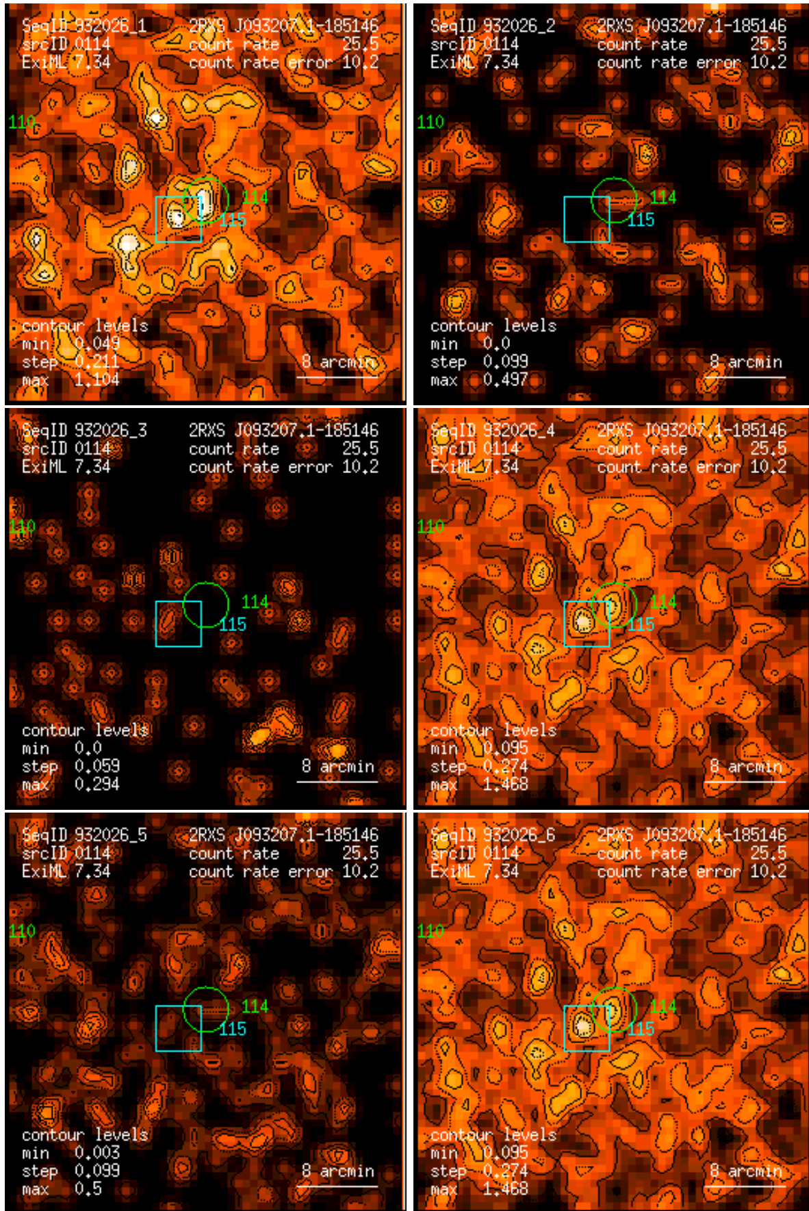
Figure 114: RASS 932026: detection 0114: band rate images, Gaussian filter: (1) PSPC channels 11 – 41, (2) 52 – 90, (3) 91 – 201, (4) 11 – 235, (5) 52 – 201, (6) 11 – 201. Broad band rates in counts/ks. Band rate contour levels in counts/ks/arcmin 2 .
