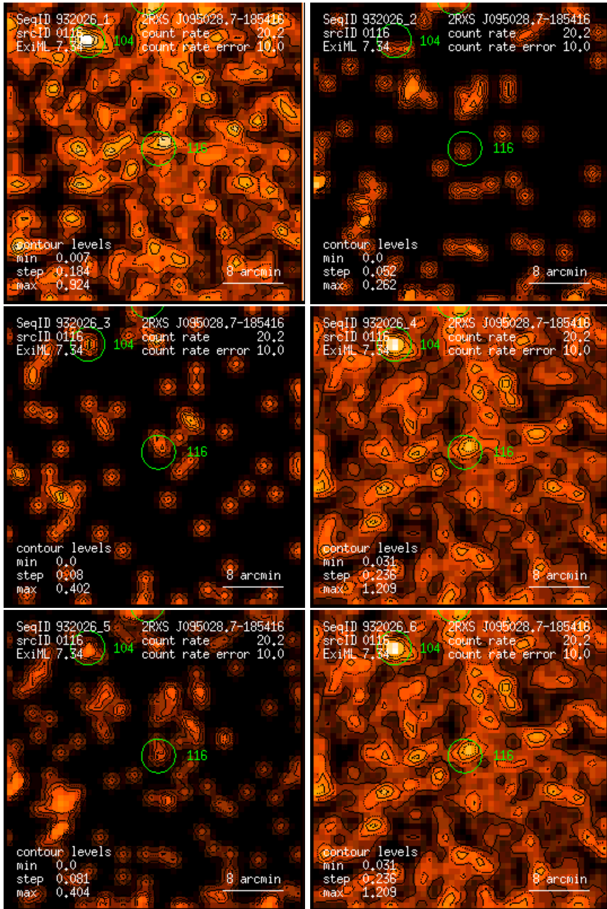
Figure 116: RASS 932026: detection 0116: band rate images, Gaussian filter: (1) PSPC channels 11 – 41, (2) 52 – 90, (3) 91 – 201, (4) 11 – 235, (5) 52 – 201, (6) 11 – 201. Broad band rates in counts/ks. Band rate contour levels in counts/ks/arcmin 2 .
