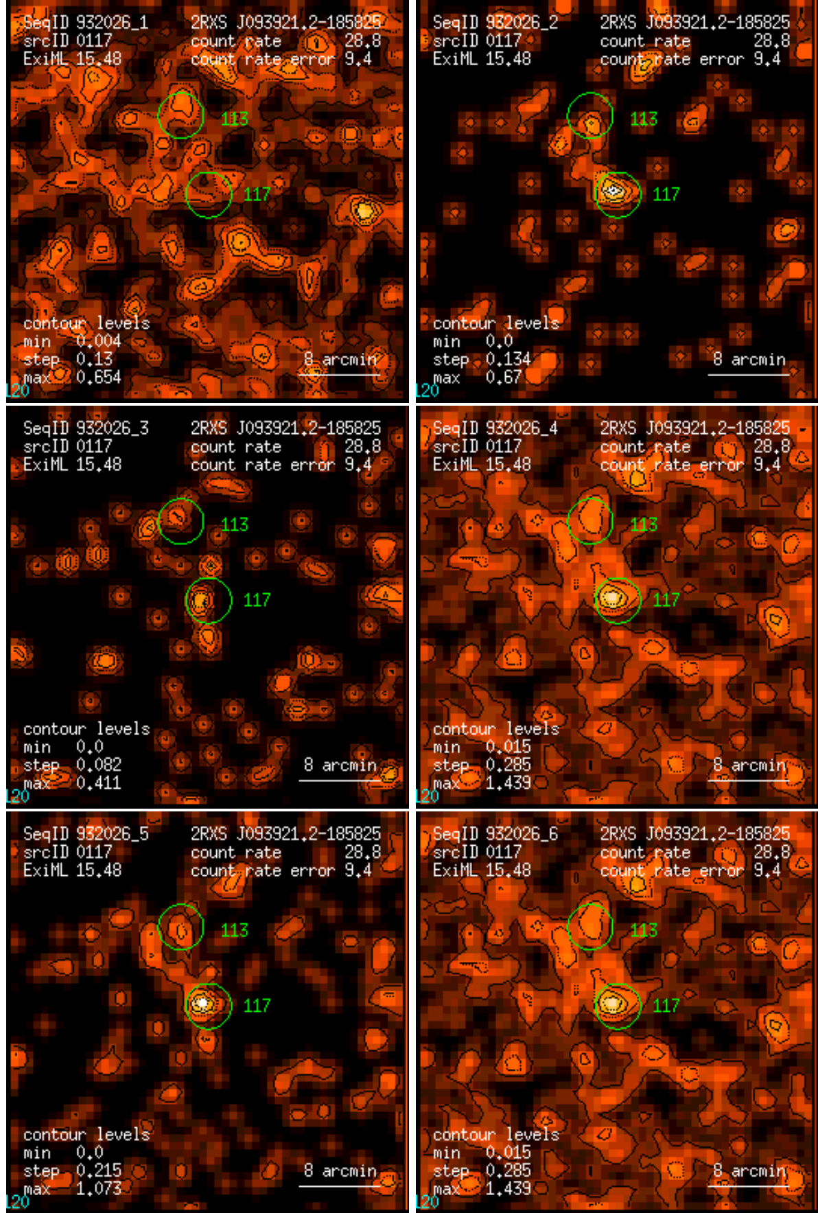
Figure 117: RASS 932026: detection 0117: band rate images, Gaussian filter: (1) PSPC channels 11 – 41, (2) 52 – 90, (3) 91 – 201, (4) 11 – 235, (5) 52 – 201, (6) 11 – 201. Broad band rates in counts/ks. Band rate contour levels in counts/ks/arcmin 2 .
