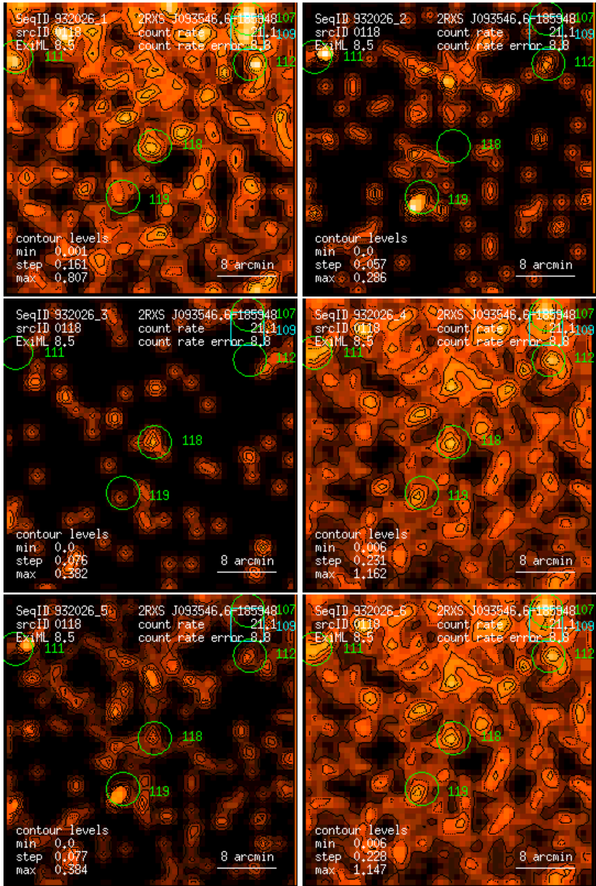
Figure 118: RASS 932026: detection 0118: band rate images, Gaussian filter: (1) PSPC channels 11 – 41, (2) 52 – 90, (3) 91 – 201, (4) 11 – 235, (5) 52 – 201, (6) 11 – 201. Broad band rates in counts/ks. Band rate contour levels in counts/ks/arcmin 2 .
