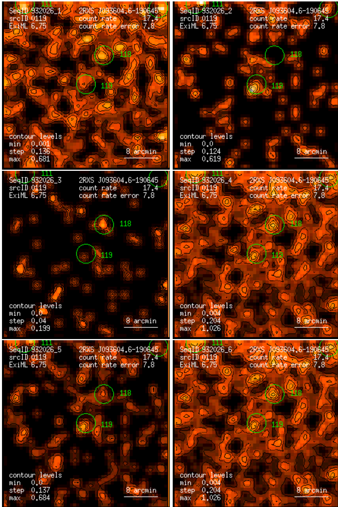
Figure 119: RASS 932026: detection 0119: band rate images, Gaussian filter: (1) PSPC channels 11 – 41, (2) 52 – 90, (3) 91 – 201, (4) 11 – 235, (5) 52 – 201, (6) 11 – 201. Broad band rates in counts/ks. Band rate contour levels in counts/ks/arcmin 2 .
