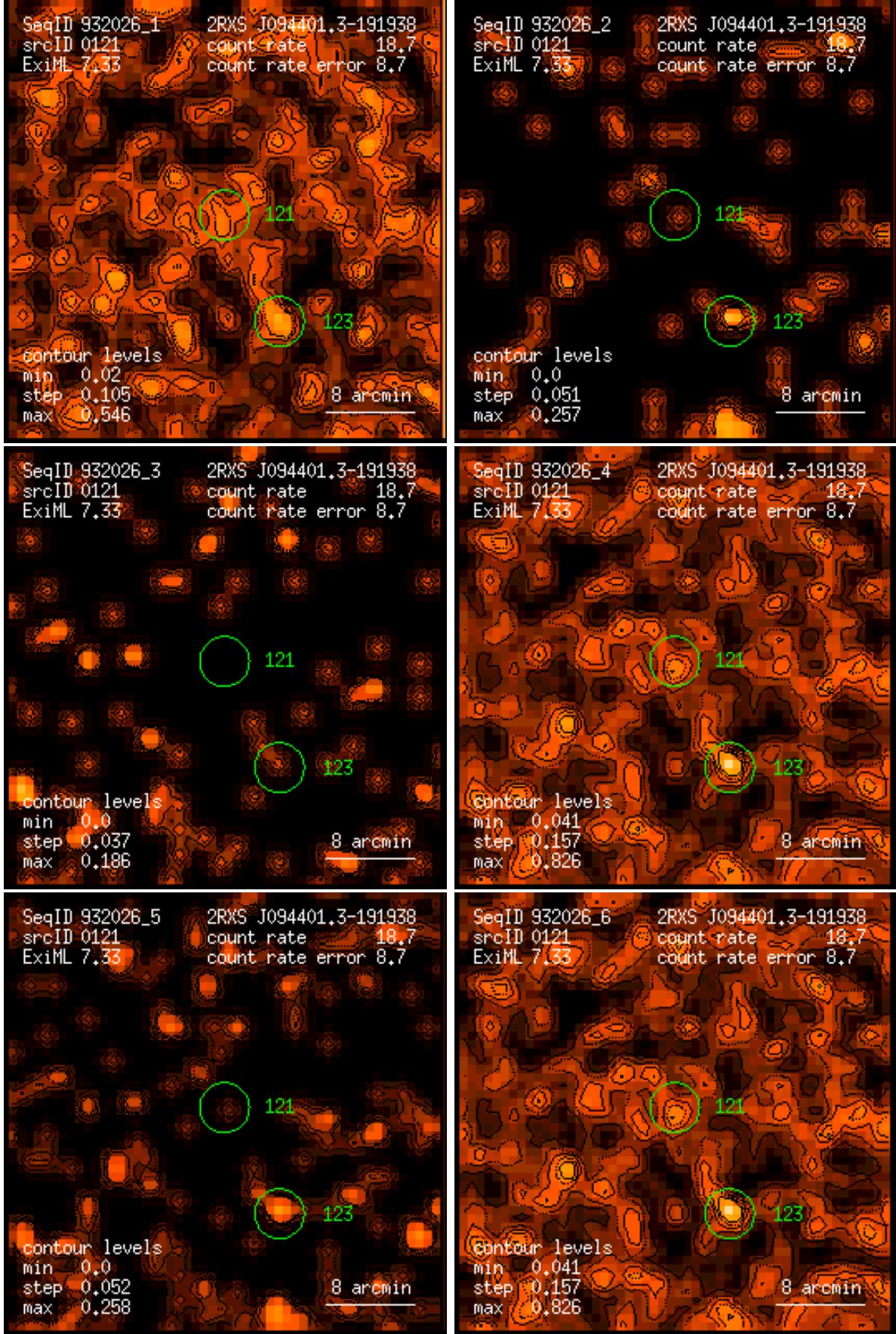
Figure 121: RASS 932026: detection 0121: band rate images, Gaussian filter: (1) PSPC channels 11 – 41, (2) 52 – 90, (3) 91 – 201, (4) 11 – 235, (5) 52 – 201, (6) 11 – 201. Broad band rates in counts/ks. Band rate contour levels in counts/ks/arcmin 2 .
