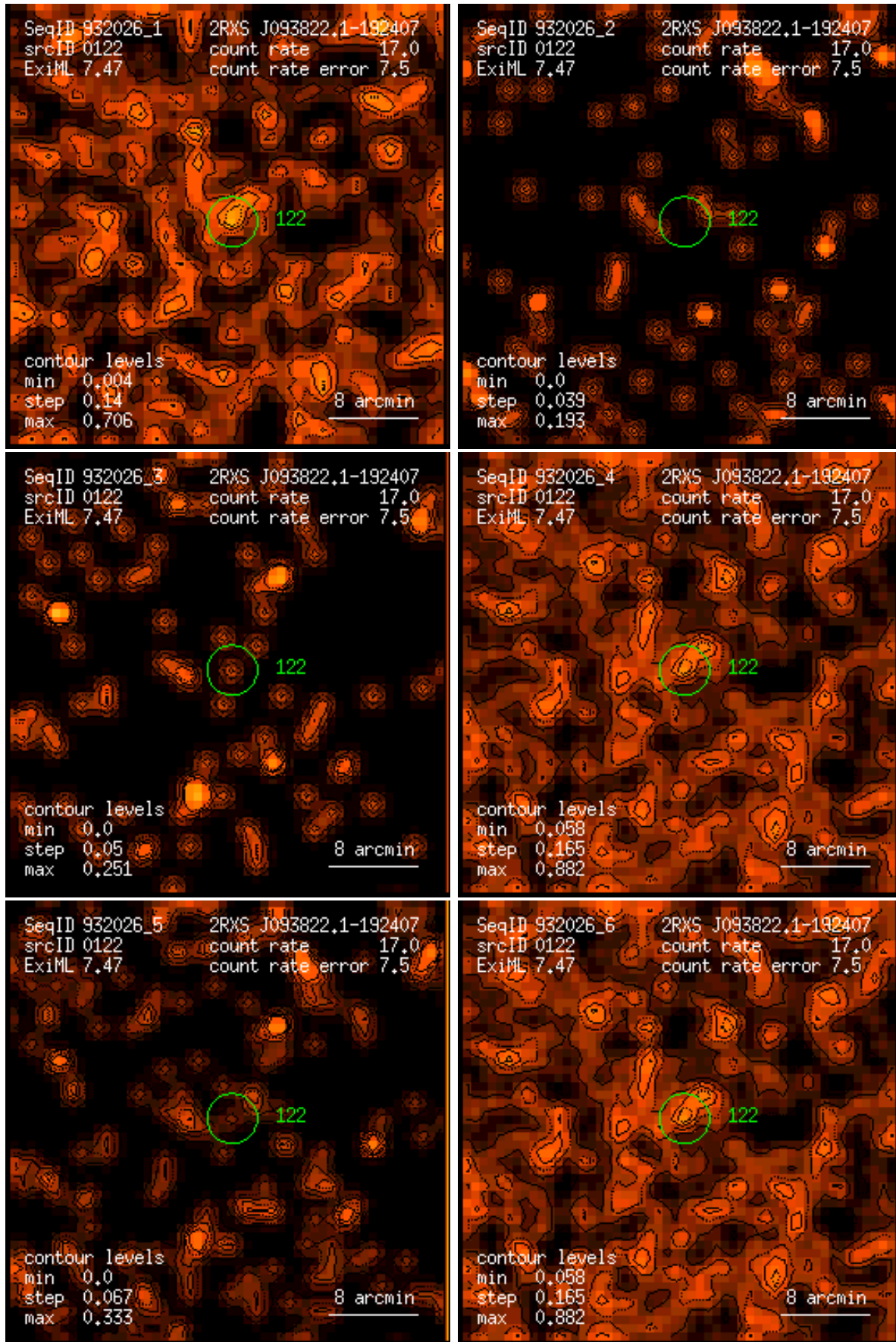
Figure 122: RASS 932026: detection 0122: band rate images, Gaussian filter: (1) PSPC channels 11 – 41, (2) 52 – 90, (3) 91 – 201, (4) 11 – 235, (5) 52 – 201, (6) 11 – 201. Broad band rates in counts/ks. Band rate contour levels in counts/ks/arcmin 2 .
