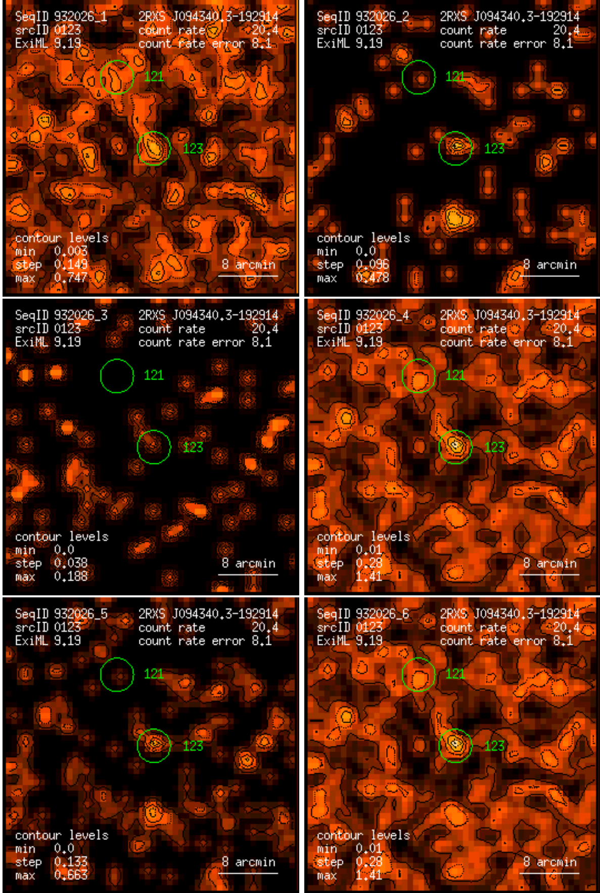
Figure 123: RASS 932026: detection 0123: band rate images, Gaussian filter: (1) PSPC channels 11 – 41, (2) 52 – 90, (3) 91 – 201, (4) 11 – 235, (5) 52 – 201, (6) 11 – 201. Broad band rates in counts/ks. Band rate contour levels in counts/ks/arcmin 2 .
