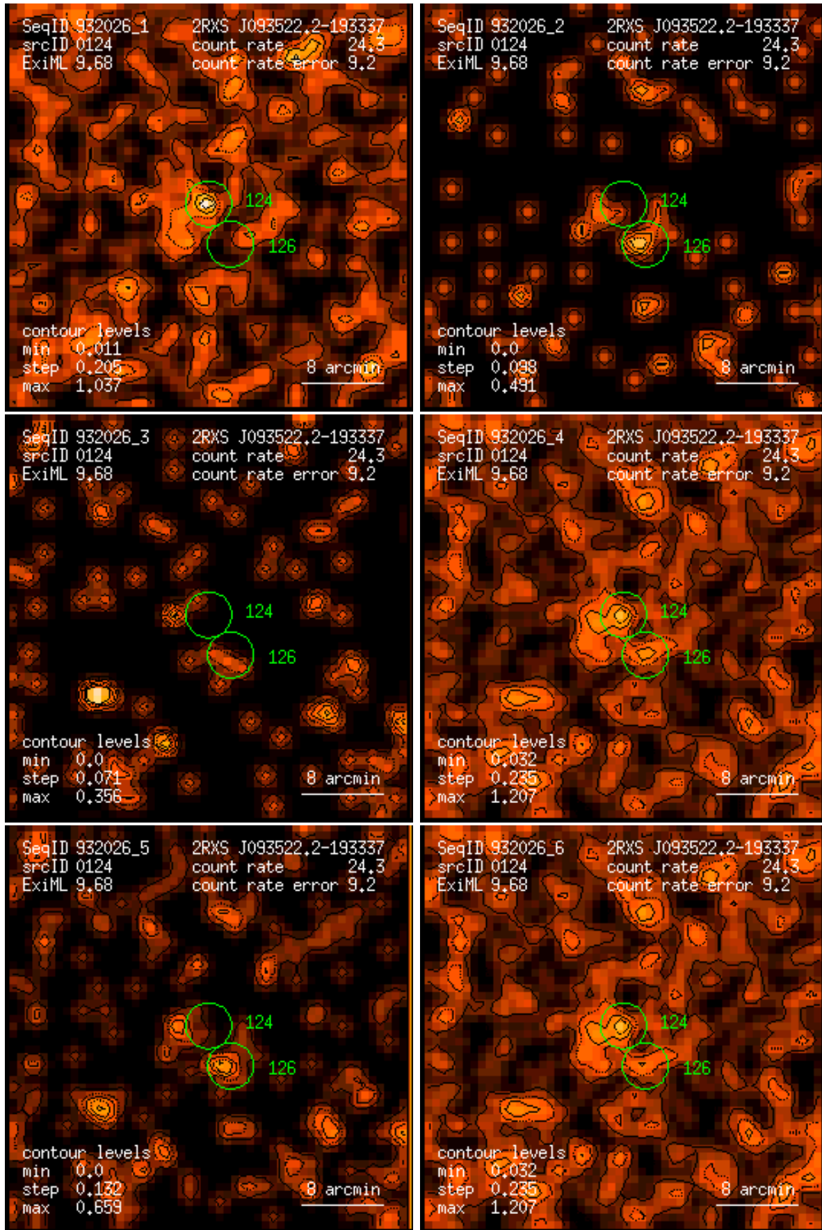
Figure 124: RASS 932026: detection 0124: band rate images, Gaussian filter: (1) PSPC channels 11 – 41, (2) 52 – 90, (3) 91 – 201, (4) 11 – 235, (5) 52 – 201, (6) 11 – 201. Broad band rates in counts/ks. Band rate contour levels in counts/ks/arcmin 2 .
