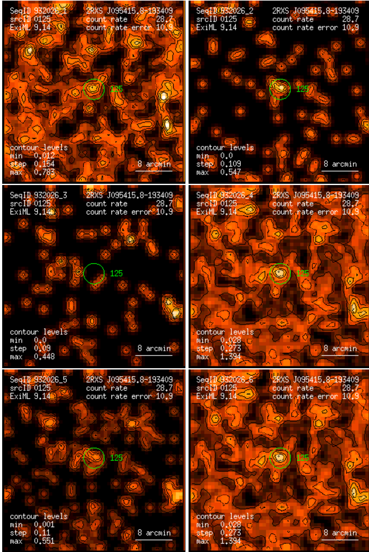
Figure 125: RASS 932026: detection 0125: band rate images, Gaussian filter: (1) PSPC channels 11 – 41, (2) 52 – 90, (3) 91 – 201, (4) 11 – 235, (5) 52 – 201, (6) 11 – 201. Broad band rates in counts/ks. Band rate contour levels in counts/ks/arcmin 2 .
