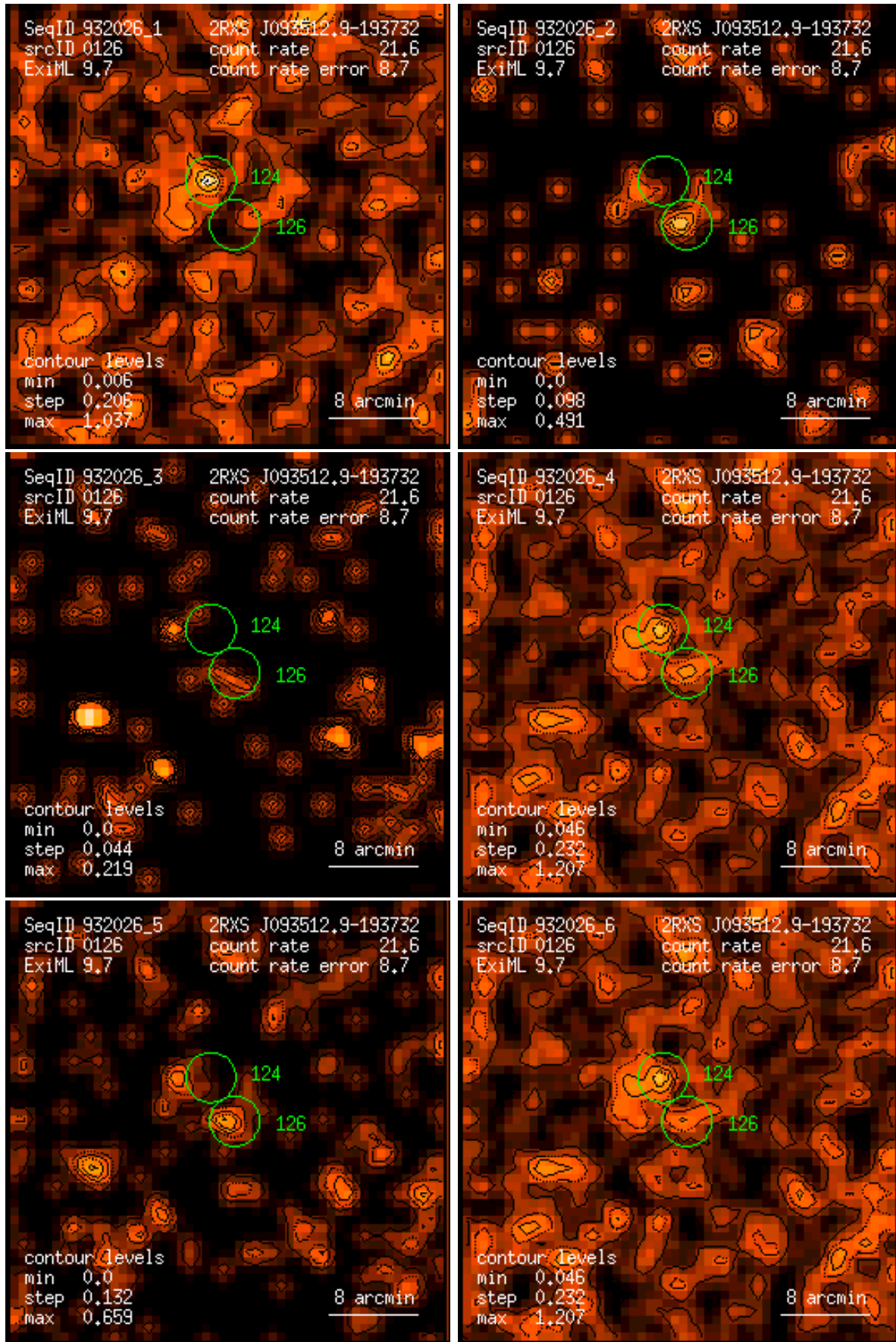
Figure 126: RASS 932026: detection 0126: band rate images, Gaussian filter: (1) PSPC channels 11 – 41, (2) 52 – 90, (3) 91 – 201, (4) 11 – 235, (5) 52 – 201, (6) 11 – 201. Broad band rates in counts/ks. Band rate contour levels in counts/ks/arcmin 2 .
