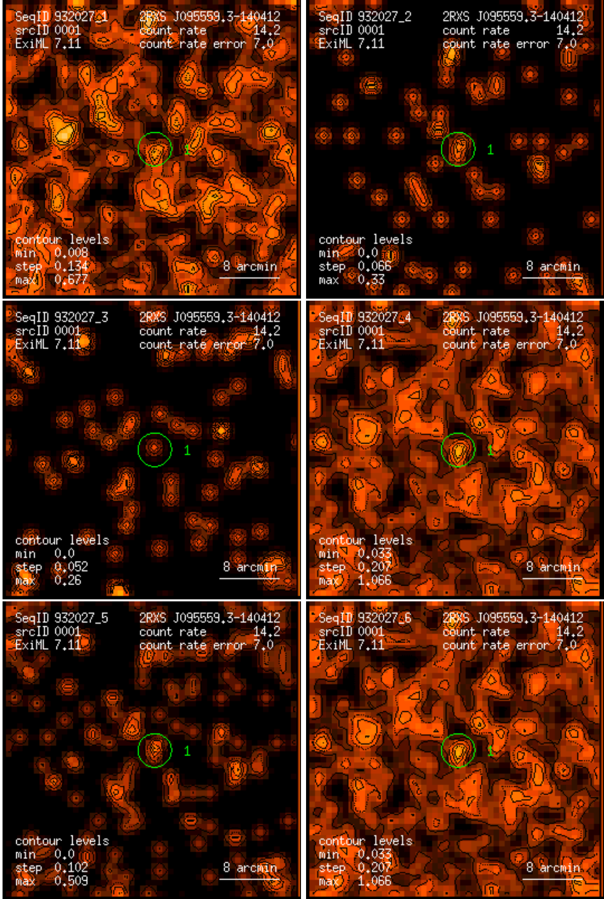
Figure 1: RASS 932027: detection 0001: band rate images, Gaussian filter: (1) PSPC channels 11 – 41, (2) 52 – 90, (3) 91 – 201, (4) 11 – 235, (5) 52 – 201, (6) 11 – 201. Broad band rates in counts/ks. Band rate contour levels in counts/ks/arcmin 2 .
