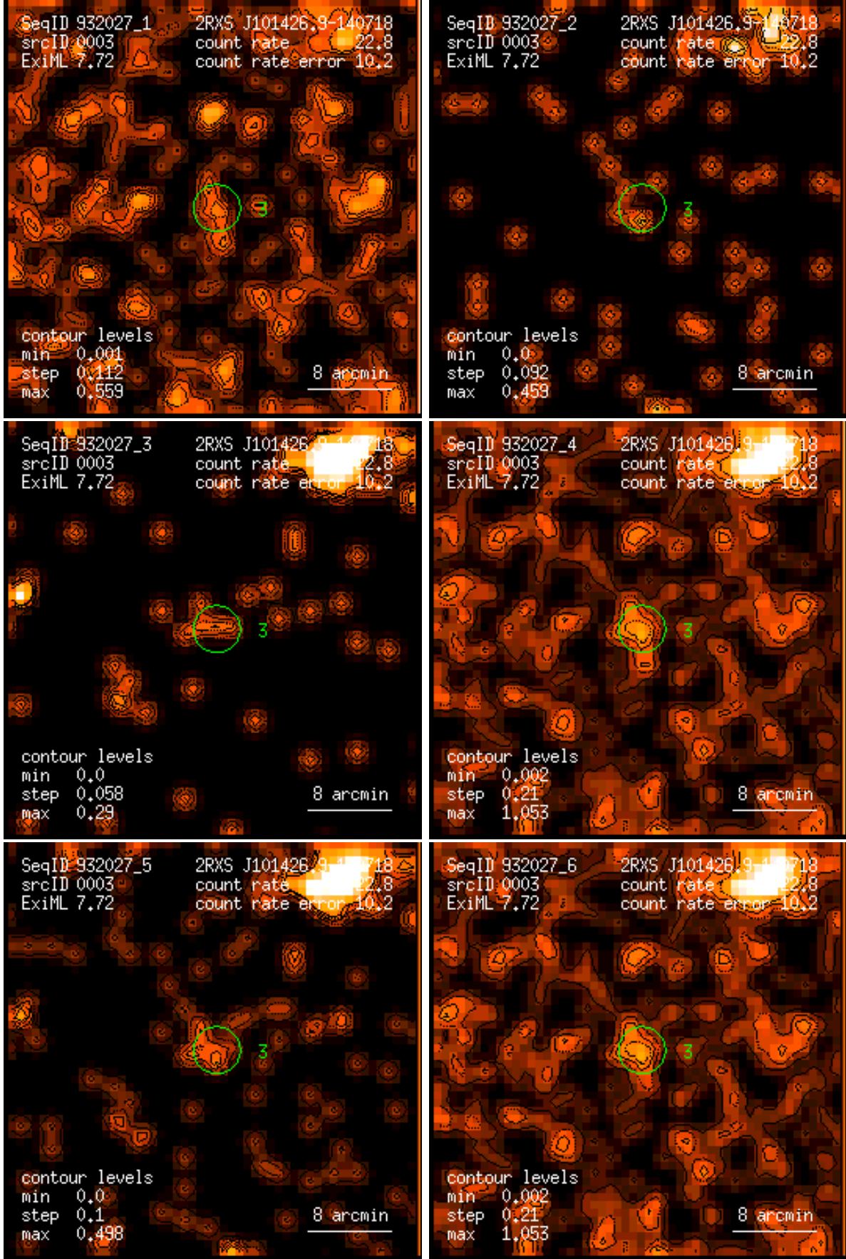
Figure 3: RASS 932027: detection 0003: band rate images, Gaussian filter: (1) PSPC channels 11 – 41, (2) 52 – 90, (3) 91 – 201, (4) 11 – 235, (5) 52 – 201, (6) 11 – 201. Broad band rates in counts/ks. Band rate contour levels in counts/ks/arcmin 2 .
