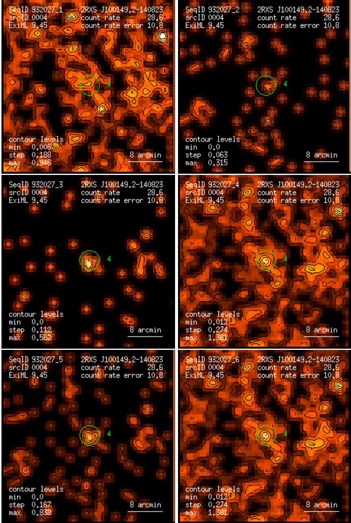
Figure 4: RASS 932027: detection 0004: band rate images, Gaussian filter: (1) PSPC channels 11 – 41, (2) 52 – 90, (3) 91 – 201, (4) 11 – 235, (5) 52 – 201, (6) 11 – 201. Broad band rates in counts/ks. Band rate contour levels in counts/ks/arcmin 2 .
