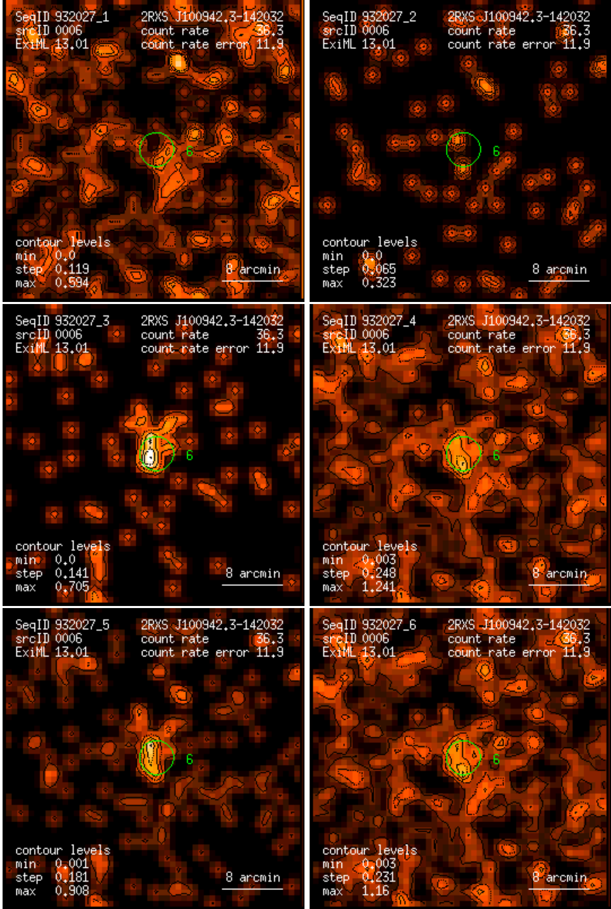
Figure 6: RASS 932027: detection 0006: band rate images, Gaussian filter: (1) PSPC channels 11 – 41, (2) 52 – 90, (3) 91 – 201, (4) 11 – 235, (5) 52 – 201, (6) 11 – 201. Broad band rates in counts/ks. Band rate contour levels in counts/ks/arcmin 2 .
