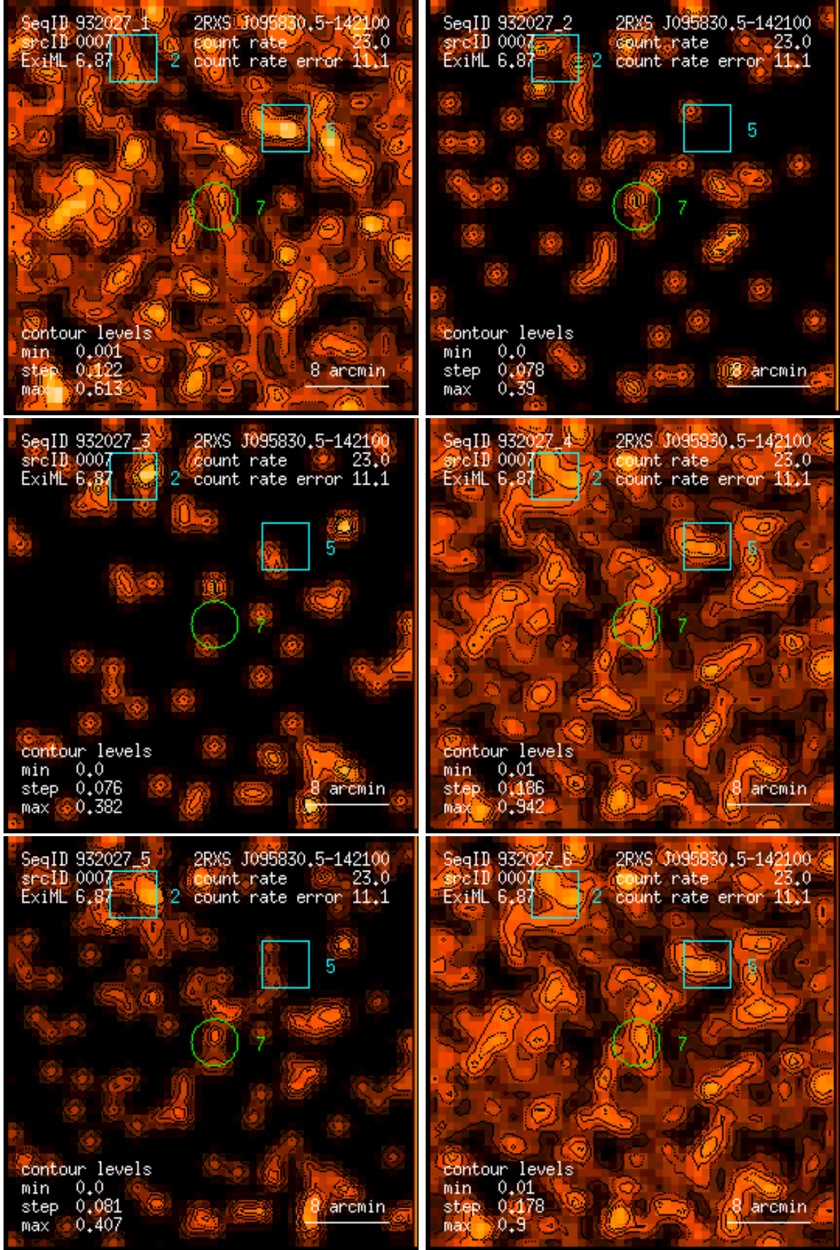
Figure 7: RASS 932027: detection 0007: band rate images, Gaussian filter: (1) PSPC channels 11 – 41, (2) 52 – 90, (3) 91 – 201, (4) 11 – 235, (5) 52 – 201, (6) 11 – 201. Broad band rates in counts/ks. Band rate contour levels in counts/ks/arcmin 2 .
