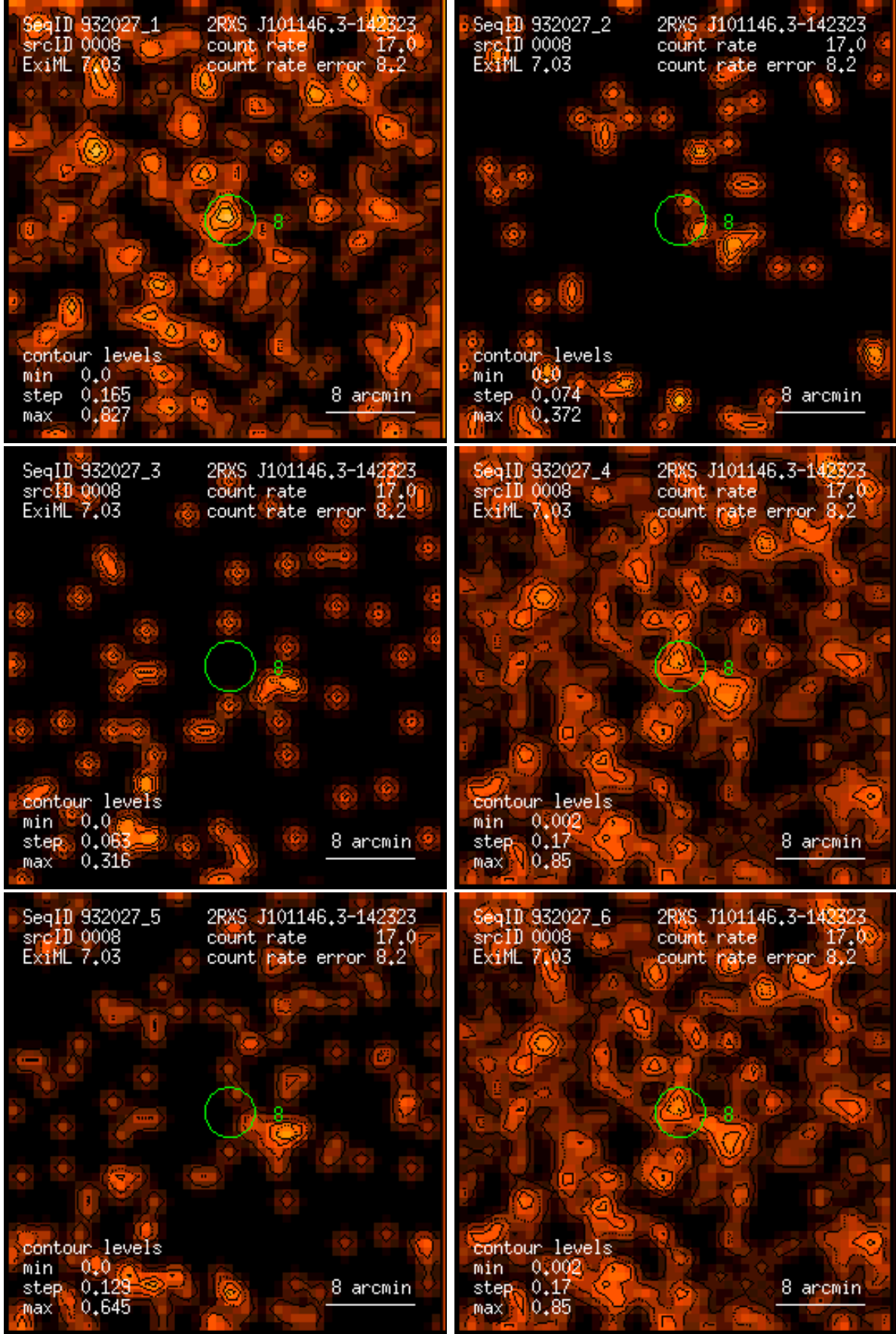
Figure 8: RASS 932027: detection 0008: band rate images, Gaussian filter: (1) PSPC channels 11 – 41, (2) 52 – 90, (3) 91 – 201, (4) 11 – 235, (5) 52 – 201, (6) 11 – 201. Broad band rates in counts/ks. Band rate contour levels in counts/ks/arcmin 2 .
