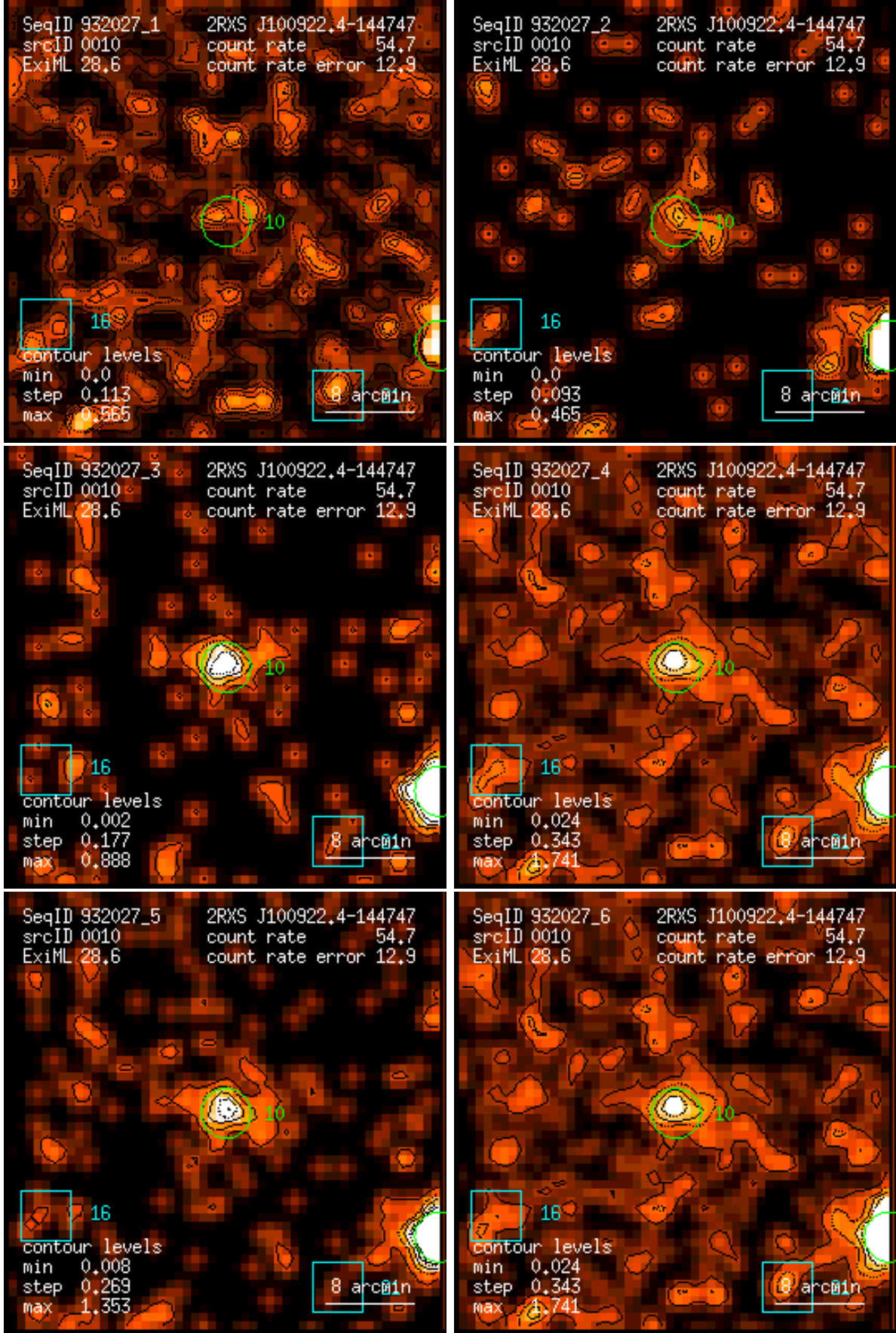
Figure 10: RASS 932027: detection 0010: band rate images, Gaussian filter: (1) PSPC channels 11 – 41, (2) 52 – 90, (3) 91 – 201, (4) 11 – 235, (5) 52 – 201, (6) 11 – 201. Broad band rates in counts/ks. Band rate contour levels in counts/ks/arcmin 2 .
