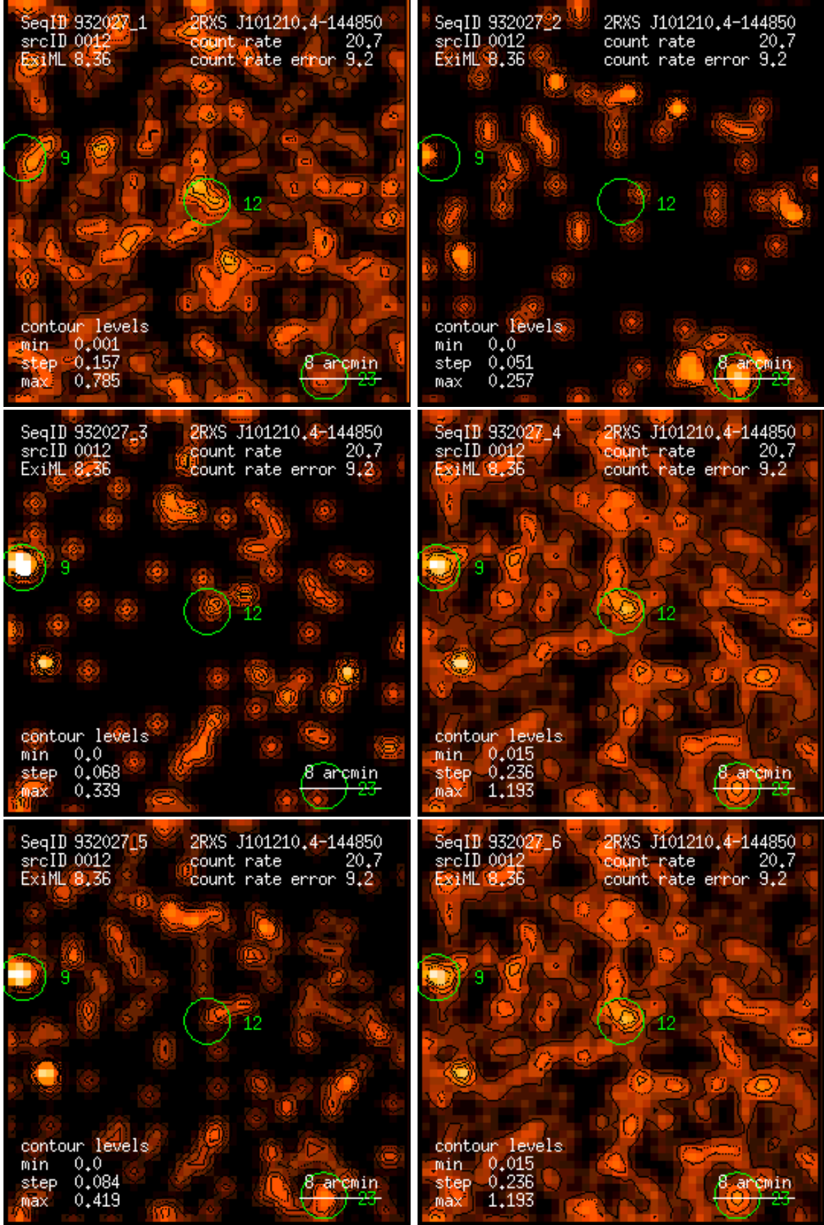
Figure 12: RASS 932027: detection 0012: band rate images, Gaussian filter: (1) PSPC channels 11 – 41, (2) 52 – 90, (3) 91 – 201, (4) 11 – 235, (5) 52 – 201, (6) 11 – 201. Broad band rates in counts/ks. Band rate contour levels in counts/ks/arcmin 2 .
