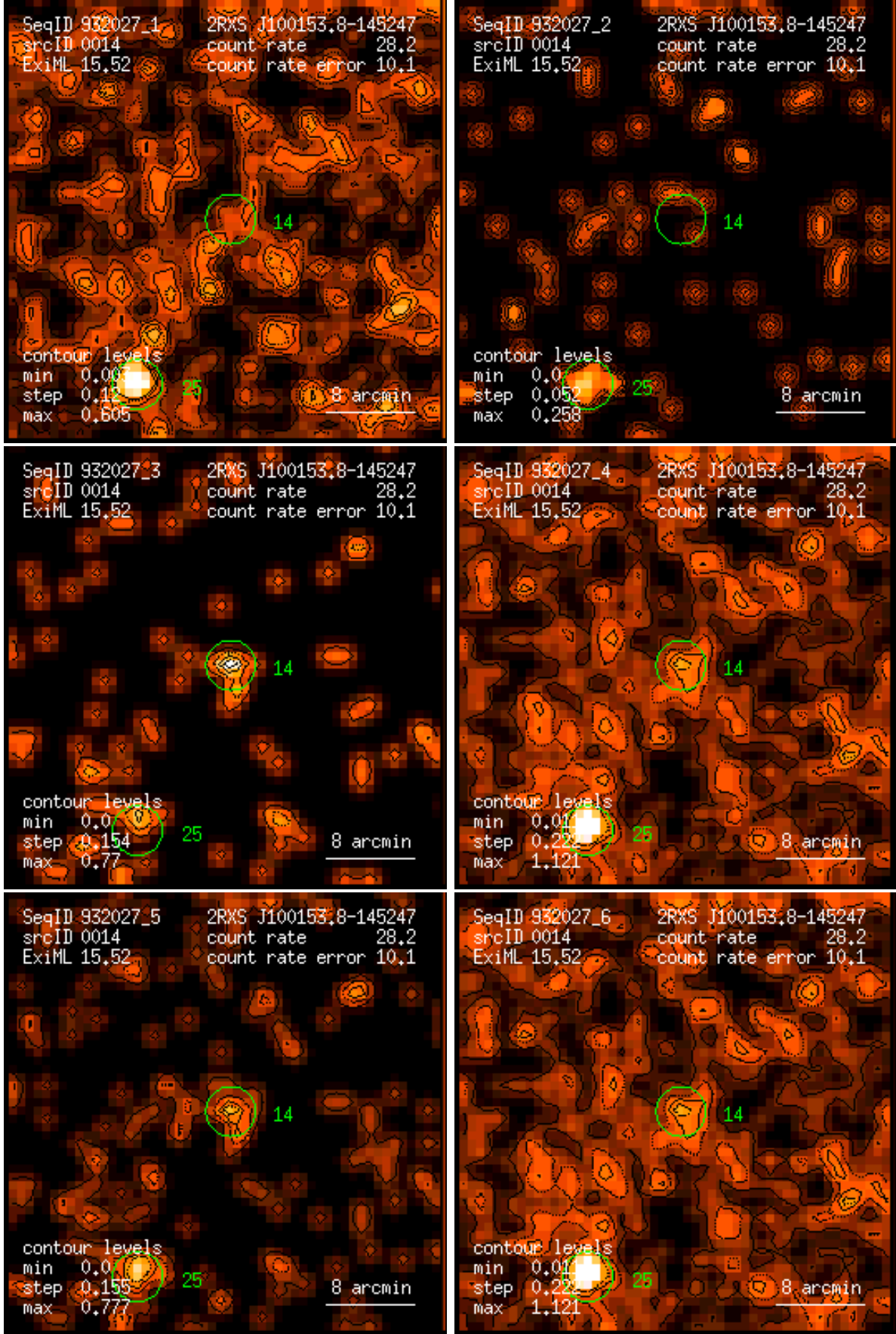
Figure 14: RASS 932027: detection 0014: band rate images, Gaussian filter: (1) PSPC channels 11 – 41, (2) 52 – 90, (3) 91 – 201, (4) 11 – 235, (5) 52 – 201, (6) 11 – 201. Broad band rates in counts/ks. Band rate contour levels in counts/ks/arcmin 2 .
