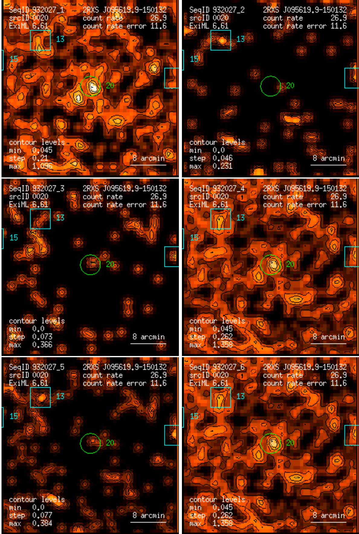
Figure 20: RASS 932027: detection 0020: band rate images, Gaussian filter: (1) PSPC channels 11 – 41, (2) 52 – 90, (3) 91 – 201, (4) 11 – 235, (5) 52 – 201, (6) 11 – 201. Broad band rates in counts/ks. Band rate contour levels in counts/ks/arcmin 2 .
