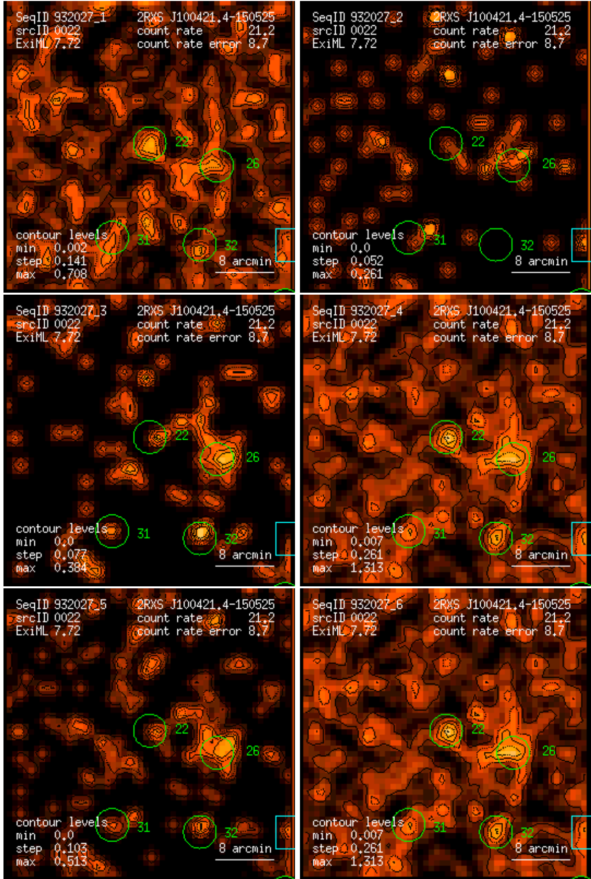
Figure 22: RASS 932027: detection 0022: band rate images, Gaussian filter: (1) PSPC channels 11 – 41, (2) 52 – 90, (3) 91 – 201, (4) 11 – 235, (5) 52 – 201, (6) 11 – 201. Broad band rates in counts/ks. Band rate contour levels in counts/ks/arcmin 2 .
