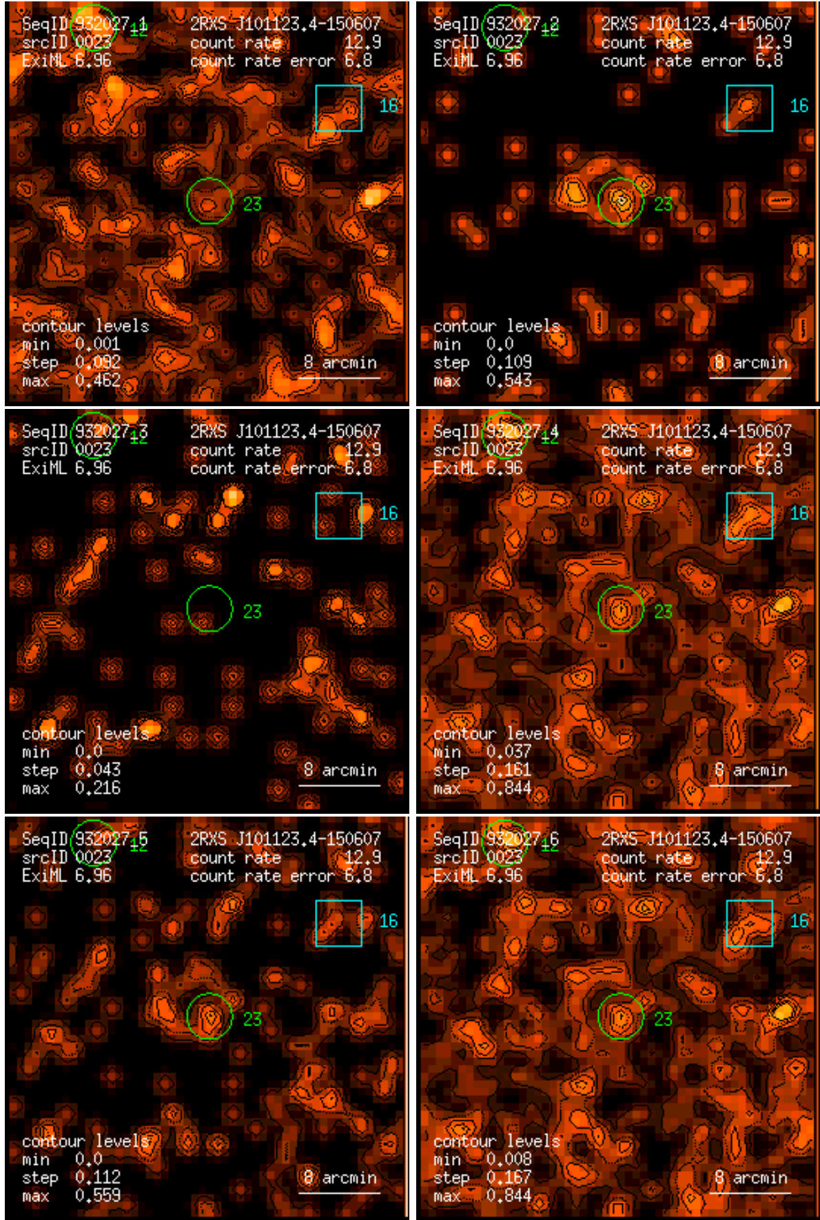
Figure 23: RASS 932027: detection 0023: band rate images, Gaussian filter: (1) PSPC channels 11 – 41, (2) 52 – 90, (3) 91 – 201, (4) 11 – 235, (5) 52 – 201, (6) 11 – 201. Broad band rates in counts/ks. Band rate contour levels in counts/ks/arcmin 2 .
