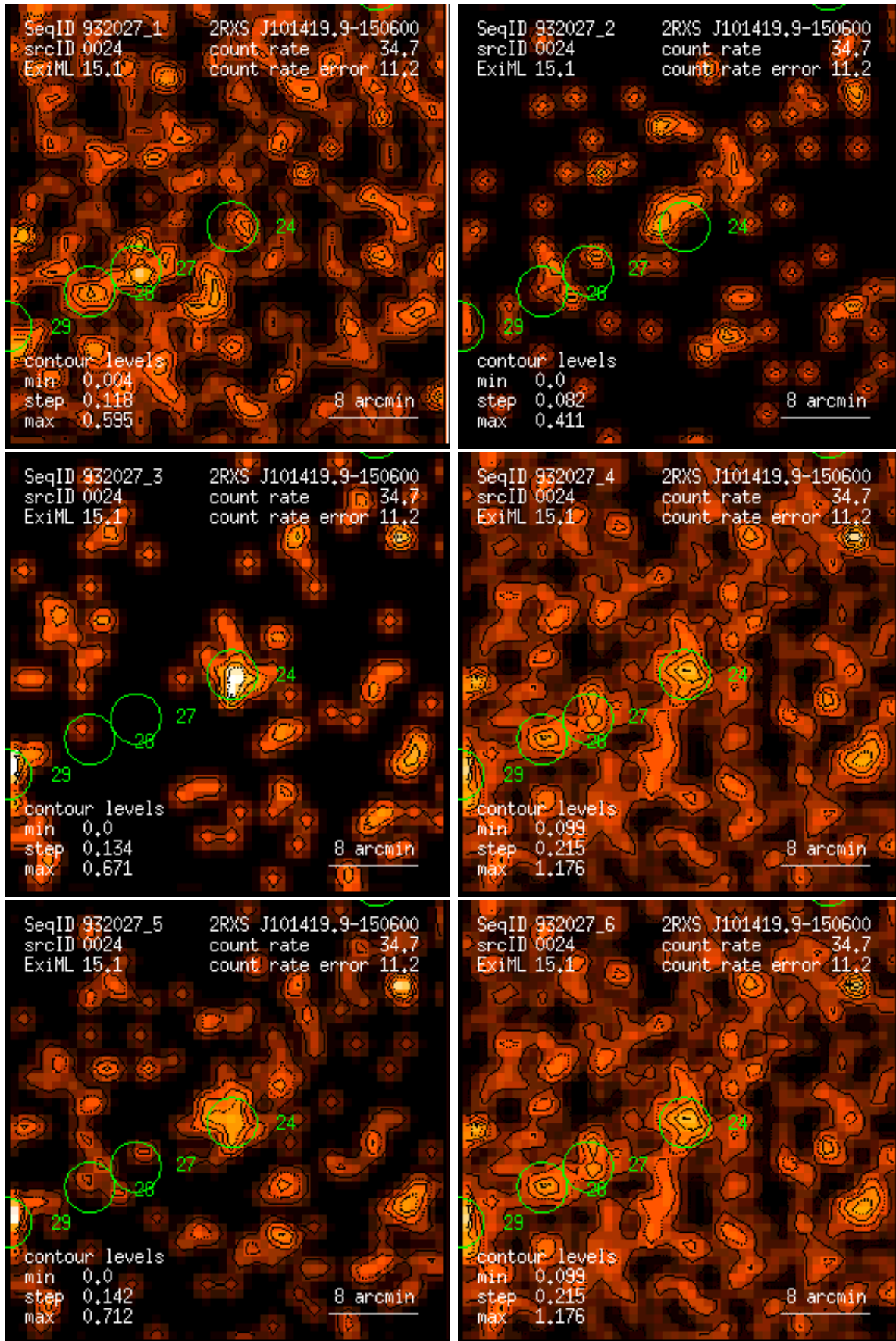
Figure 24: RASS 932027: detection 0024: band rate images, Gaussian filter: (1) PSPC channels 11 – 41, (2) 52 – 90, (3) 91 – 201, (4) 11 – 235, (5) 52 – 201, (6) 11 – 201. Broad band rates in counts/ks. Band rate contour levels in counts/ks/arcmin 2 .
