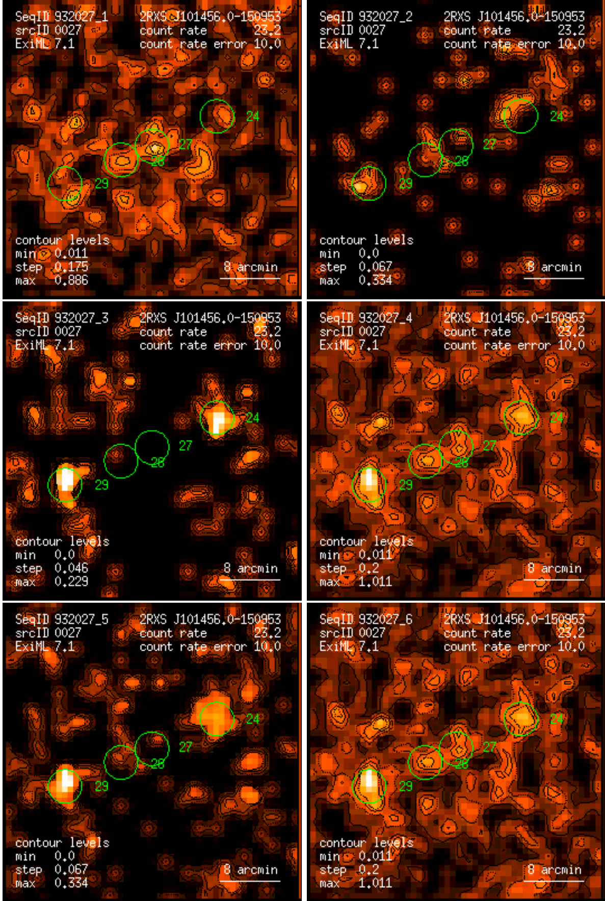
Figure 27: RASS 932027: detection 0027: band rate images, Gaussian filter: (1) PSPC channels 11 – 41, (2) 52 – 90, (3) 91 – 201, (4) 11 – 235, (5) 52 – 201, (6) 11 – 201. Broad band rates in counts/ks. Band rate contour levels in counts/ks/arcmin 2 .
