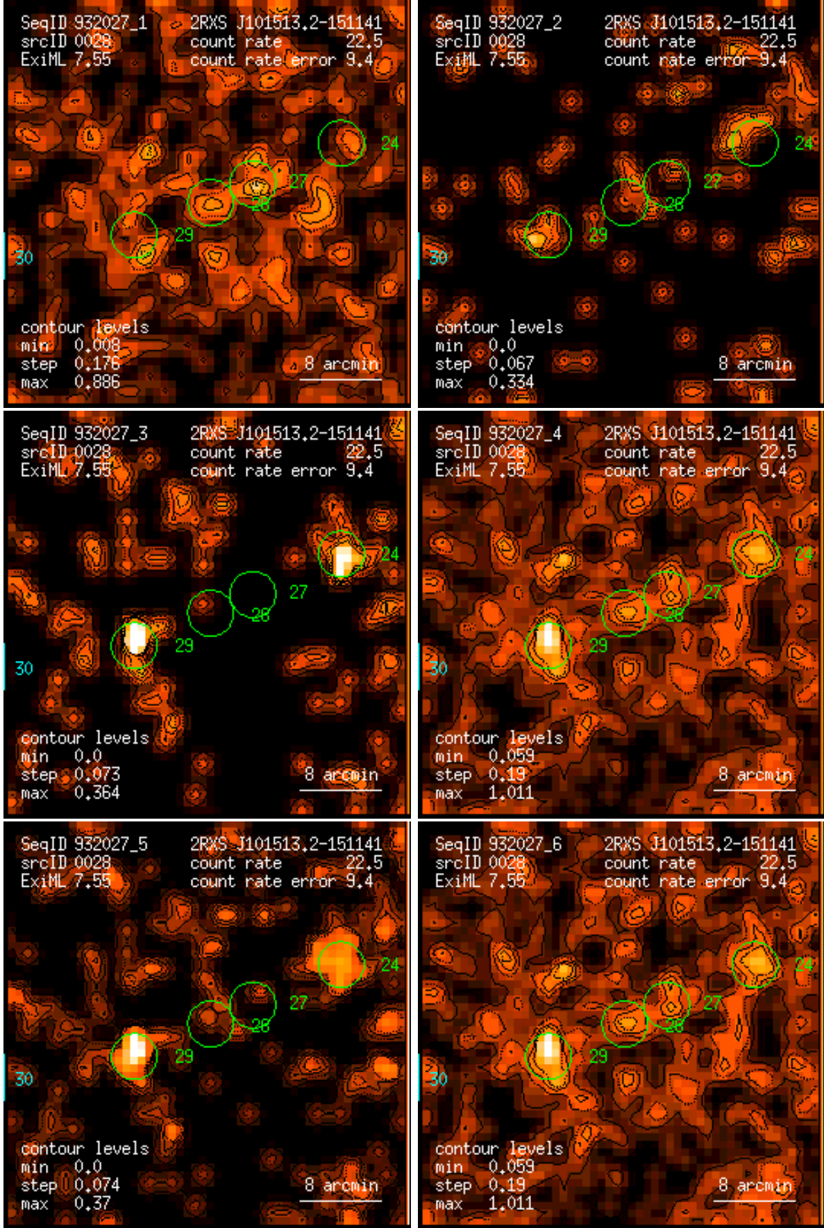
Figure 28: RASS 932027: detection 0028: band rate images, Gaussian filter: (1) PSPC channels 11 – 41, (2) 52 – 90, (3) 91 – 201, (4) 11 – 235, (5) 52 – 201, (6) 11 – 201. Broad band rates in counts/ks. Band rate contour levels in counts/ks/arcmin 2 .
