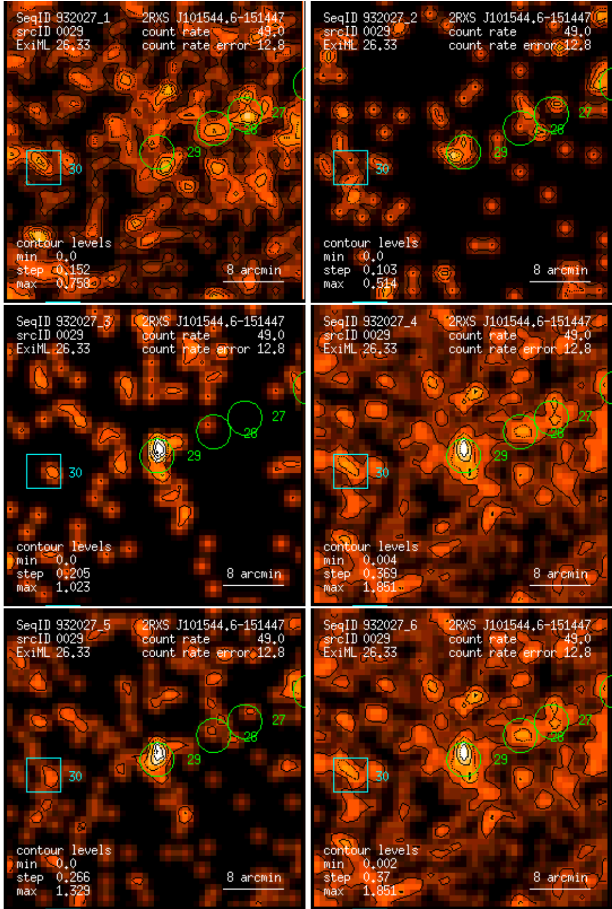
Figure 29: RASS 932027: detection 0029: band rate images, Gaussian filter: (1) PSPC channels 11 – 41, (2) 52 – 90, (3) 91 – 201, (4) 11 – 235, (5) 52 – 201, (6) 11 – 201. Broad band rates in counts/ks. Band rate contour levels in counts/ks/arcmin 2 .
