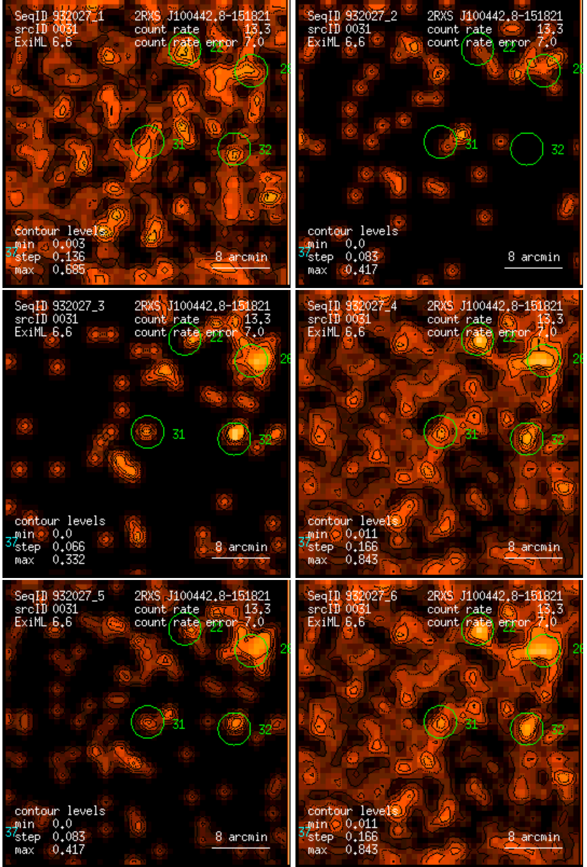
Figure 31: RASS 932027: detection 0031: band rate images, Gaussian filter: (1) PSPC channels 11 – 41, (2) 52 – 90, (3) 91 – 201, (4) 11 – 235, (5) 52 – 201, (6) 11 – 201. Broad band rates in counts/ks. Band rate contour levels in counts/ks/arcmin 2 .
