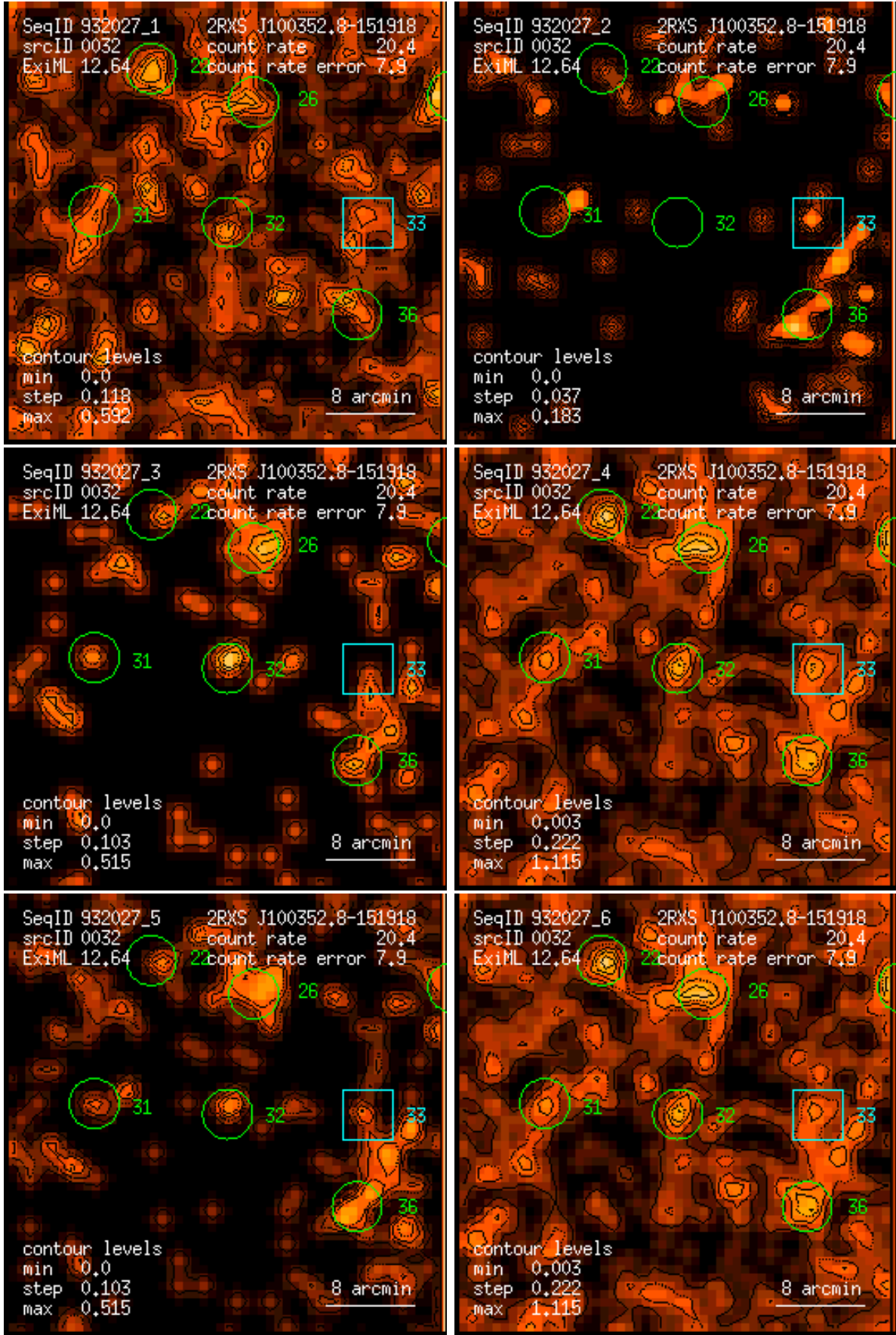
Figure 32: RASS 932027: detection 0032: band rate images, Gaussian filter: (1) PSPC channels 11 – 41, (2) 52 – 90, (3) 91 – 201, (4) 11 – 235, (5) 52 – 201, (6) 11 – 201. Broad band rates in counts/ks. Band rate contour levels in counts/ks/arcmin 2 .
