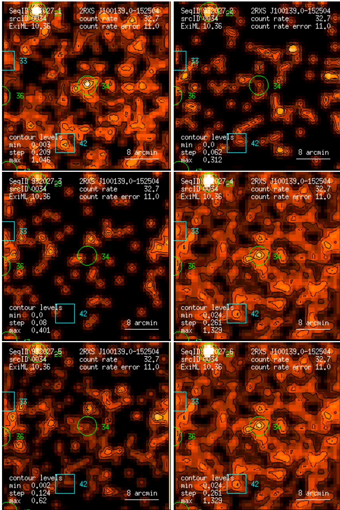
Figure 34: RASS 932027: detection 0034: band rate images, Gaussian filter: (1) PSPC channels 11 – 41, (2) 52 – 90, (3) 91 – 201, (4) 11 – 235, (5) 52 – 201, (6) 11 – 201. Broad band rates in counts/ks. Band rate contour levels in counts/ks/arcmin 2 .
