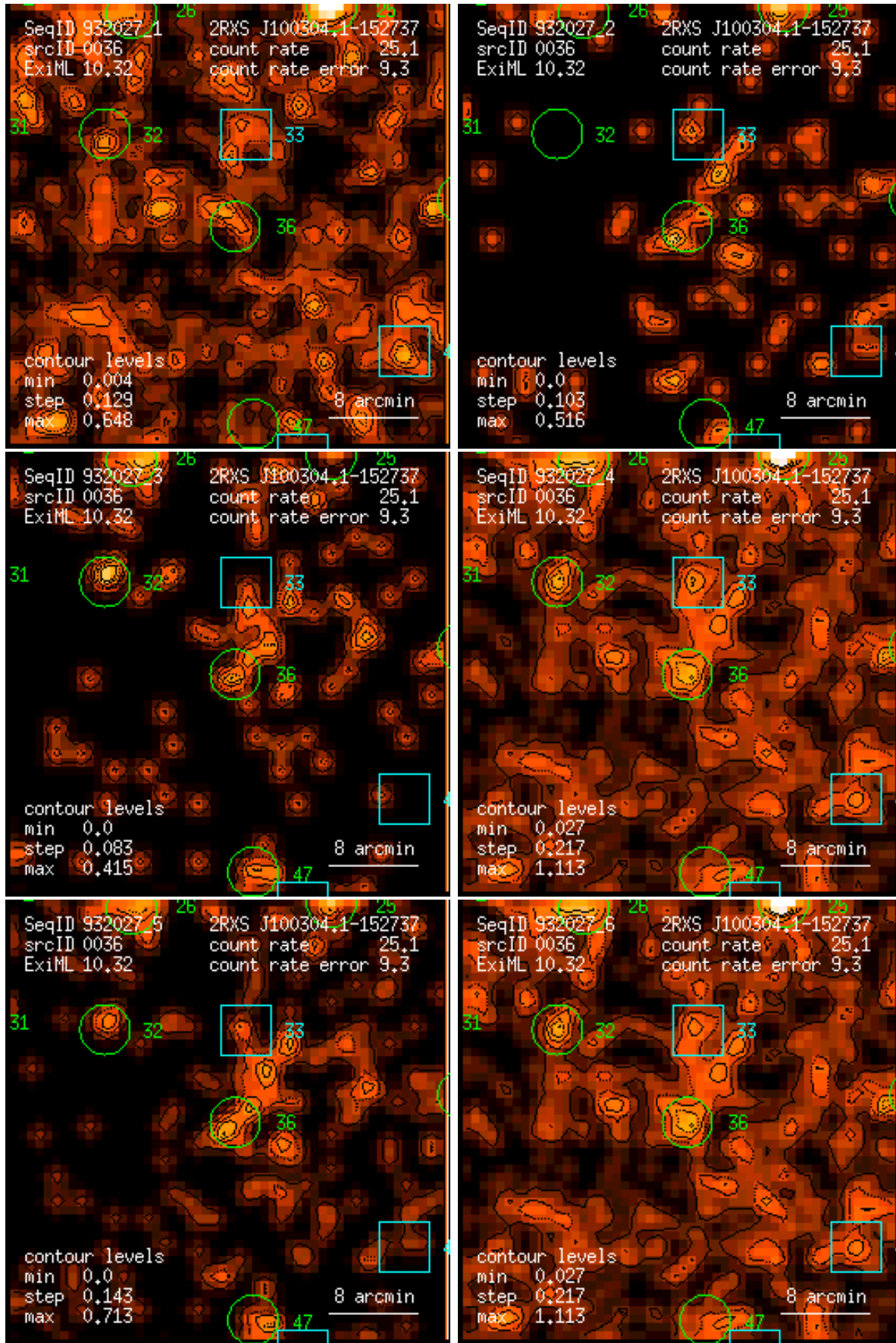
Figure 36: RASS 932027: detection 0036: band rate images, Gaussian filter: (1) PSPC channels 11 – 41, (2) 52 – 90, (3) 91 – 201, (4) 11 – 235, (5) 52 – 201, (6) 11 – 201. Broad band rates in counts/ks. Band rate contour levels in counts/ks/arcmin 2 .
