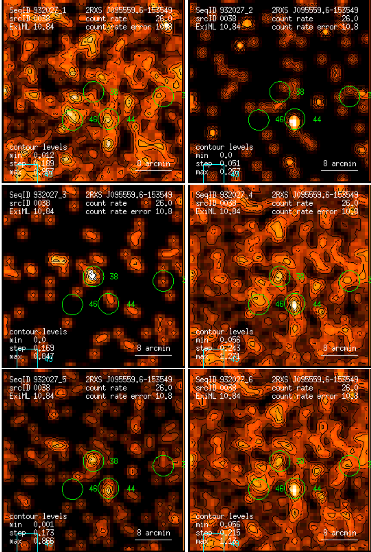
Figure 38: RASS 932027: detection 0038: band rate images, Gaussian filter: (1) PSPC channels 11 – 41, (2) 52 – 90, (3) 91 – 201, (4) 11 – 235, (5) 52 – 201, (6) 11 – 201. Broad band rates in counts/ks. Band rate contour levels in counts/ks/arcmin 2 .
