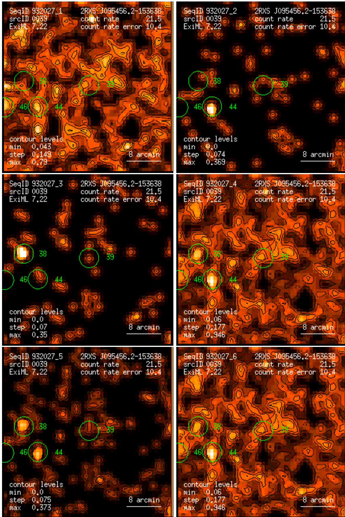
Figure 39: RASS 932027: detection 0039: band rate images, Gaussian filter: (1) PSPC channels 11 – 41, (2) 52 – 90, (3) 91 – 201, (4) 11 – 235, (5) 52 – 201, (6) 11 – 201. Broad band rates in counts/ks. Band rate contour levels in counts/ks/arcmin 2 .
