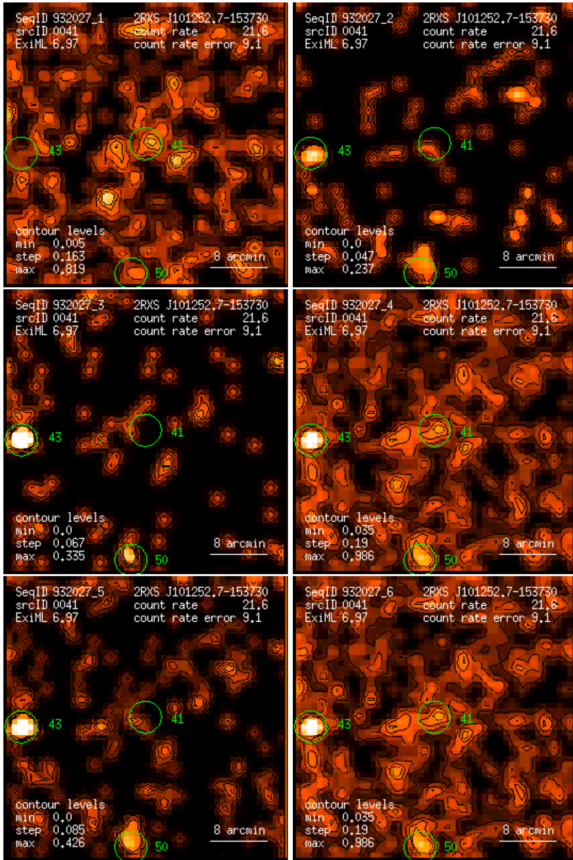
Figure 41: RASS 932027: detection 0041: band rate images, Gaussian filter: (1) PSPC channels 11 – 41, (2) 52 – 90, (3) 91 – 201, (4) 11 – 235, (5) 52 – 201, (6) 11 – 201. Broad band rates in counts/ks. Band rate contour levels in counts/ks/arcmin 2 .
